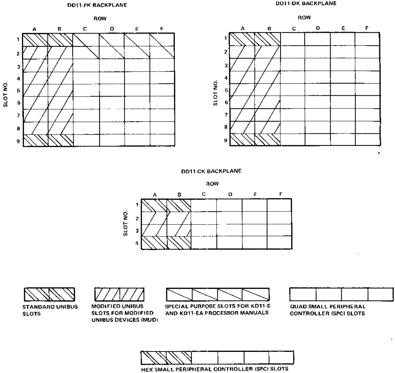
Figure 4-1 PDP-11/34 Backplanes
