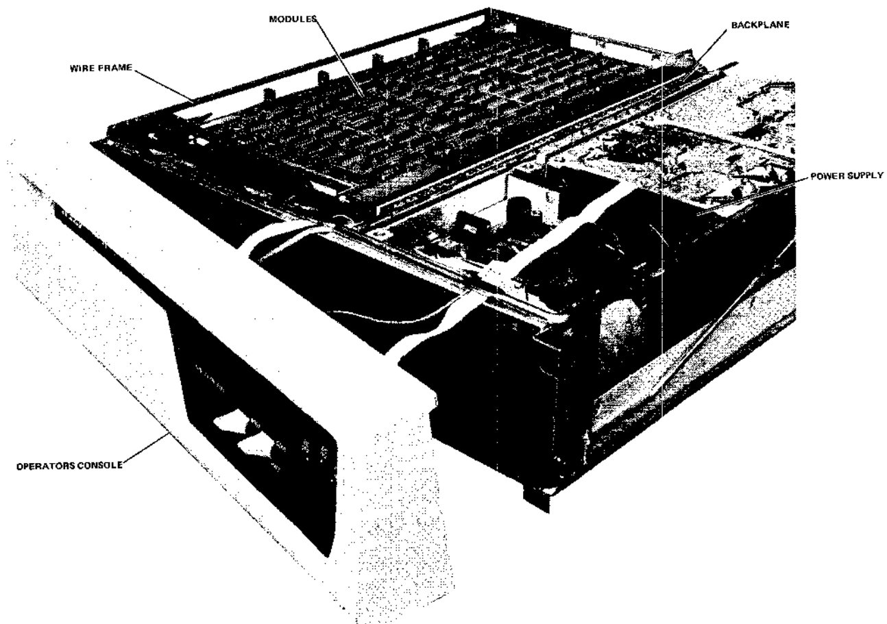
Figure 5-6 Computer Subassemblies of BA11-L Mounting Box
