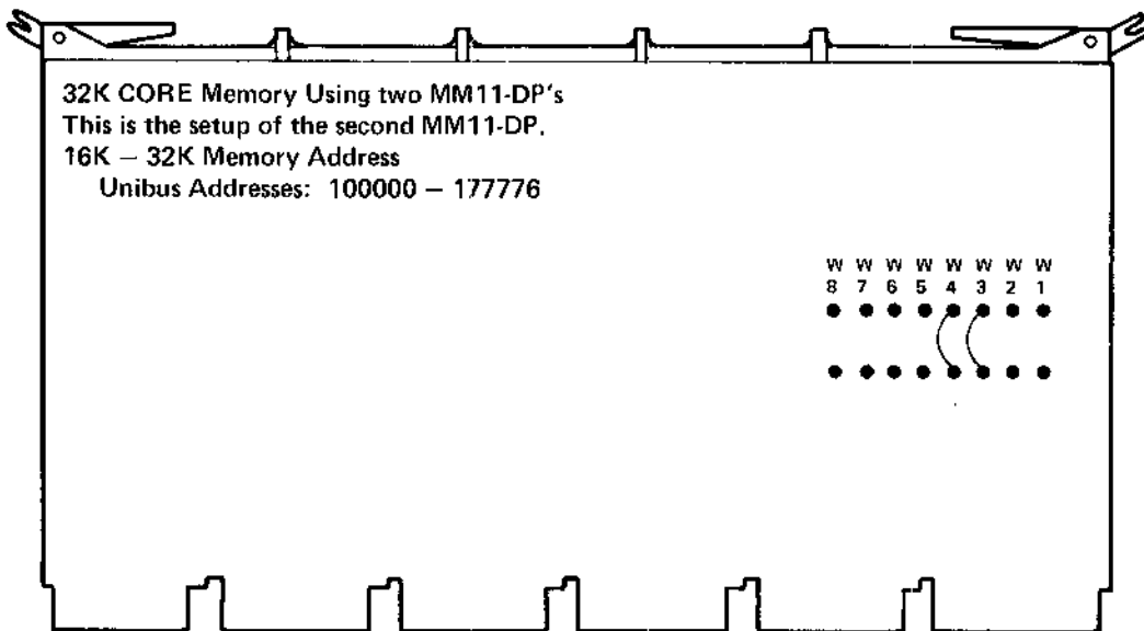
Figure 5-9 Typical Jumper Placement and Switch Settings of Modules (Sheet 8 of 9)
