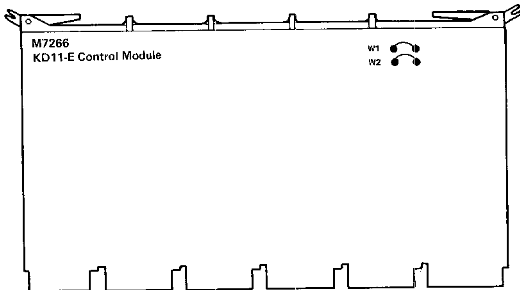
Figure 5-9 Typical Jumper Placement and Switch Settings of Modules (Sheet 2 of 9)
