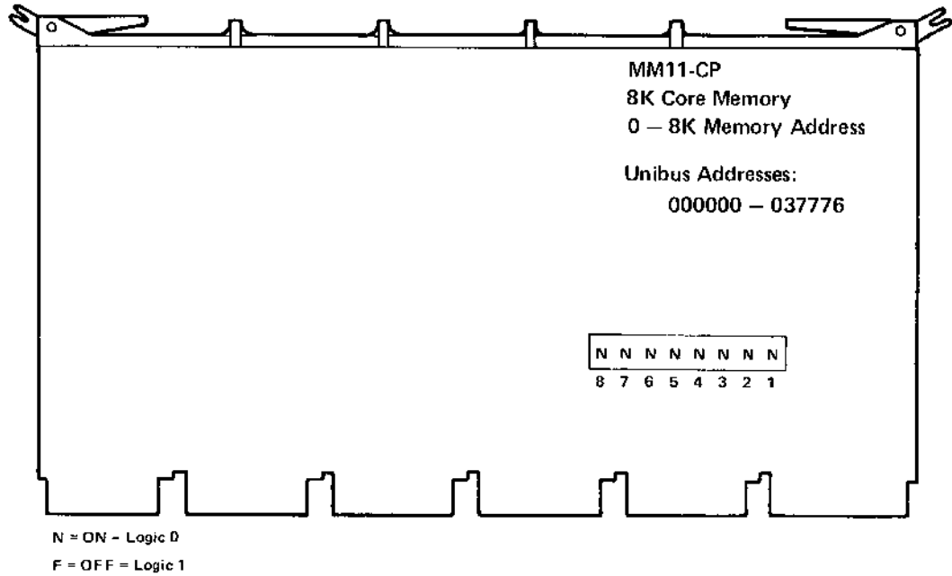
Figure 5-9 Typical Jumper Placement and Switch Settings of Modules (Sheet 7 of 9)
