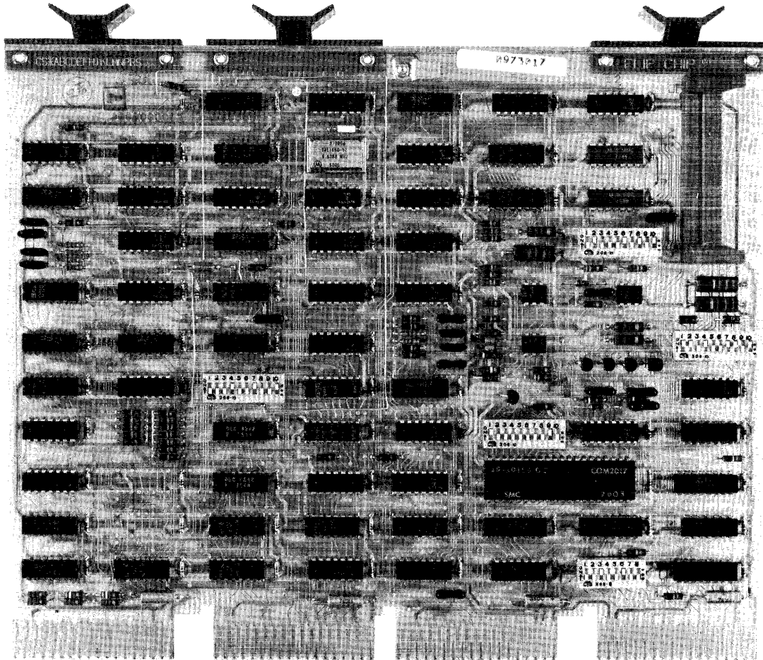
Figure 4-9 DL11-W (M7856) Switch Locations
