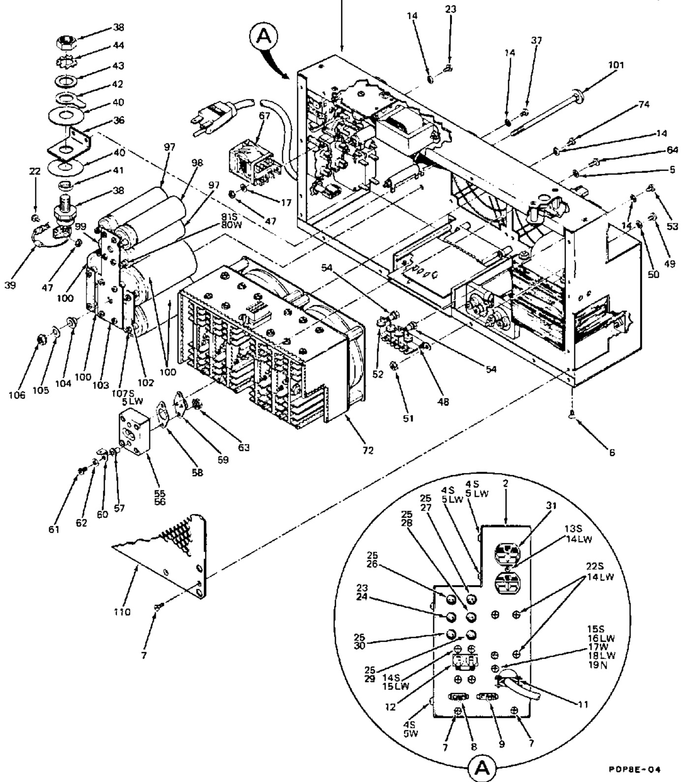
Figure 4. H724/H724A Power Supply Assembly (Sheet 1 of 2)
