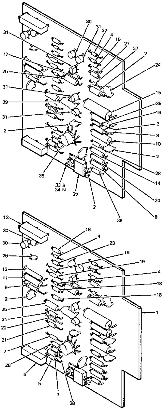
Figure 68. A-2 Control Board Assembly (Etch Rev E)
