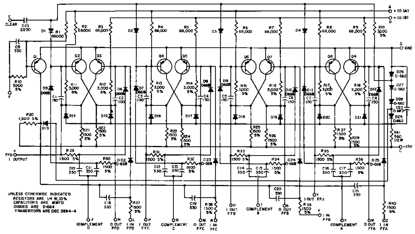
4-Bit Counter RS-4215
