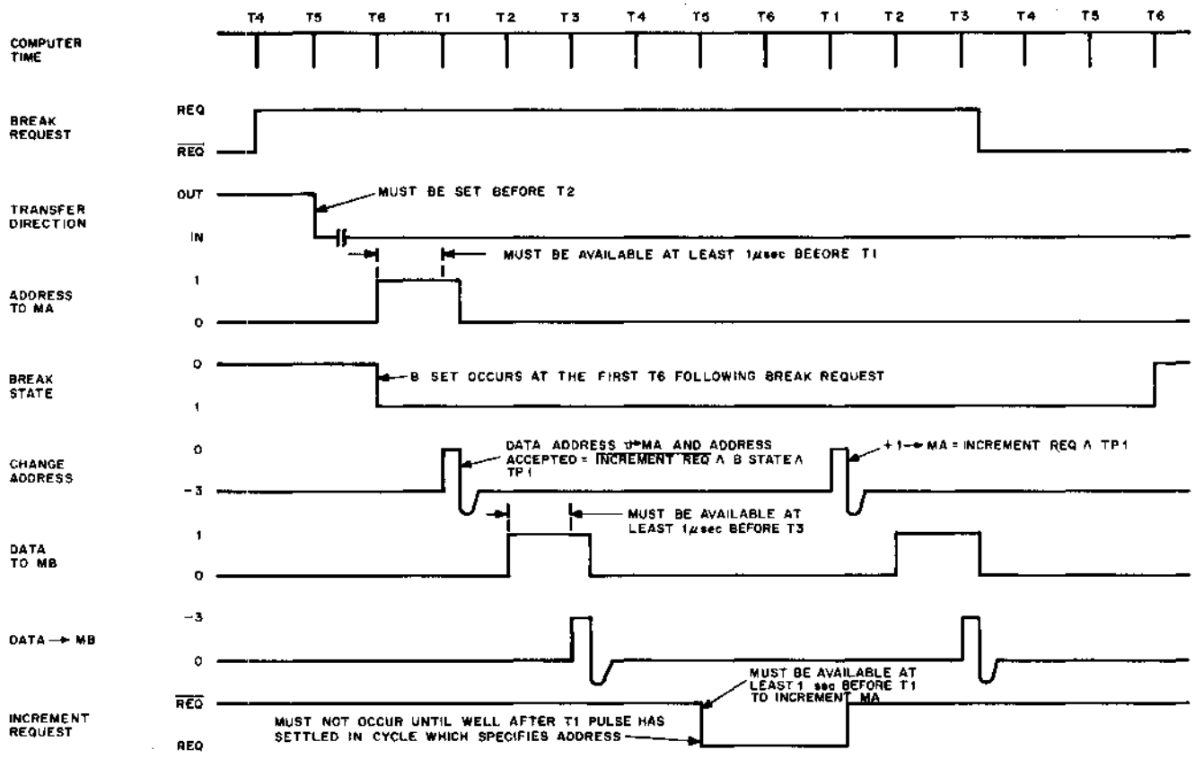
Figure 5-1 Data Break Timing
