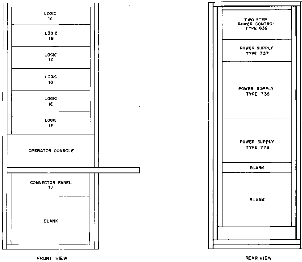
Figure 1-4 Component Locations
