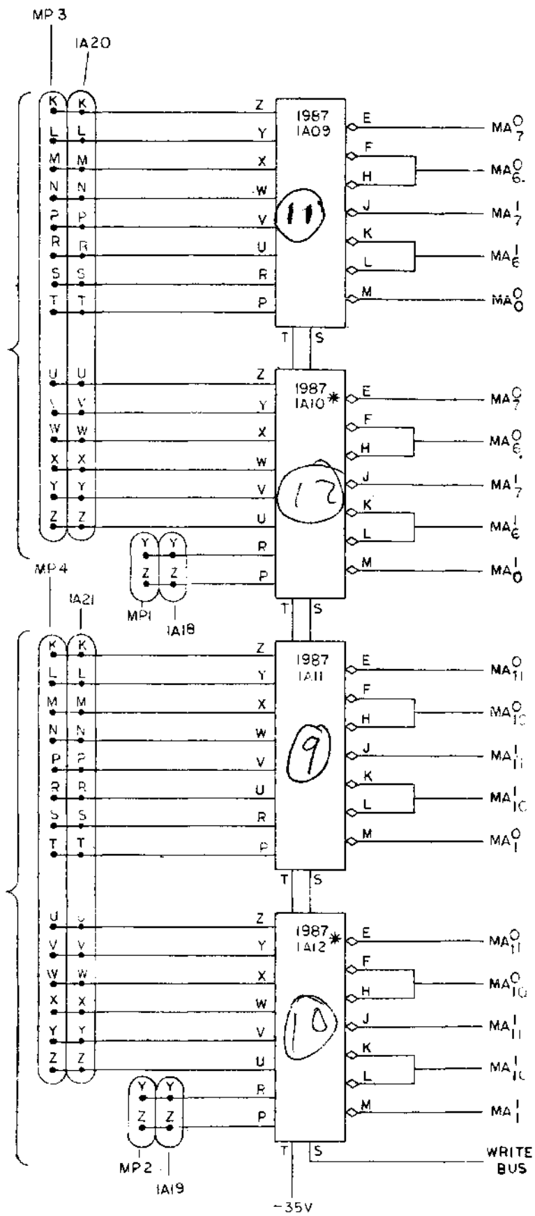
Memory "X" and "Y" Selection BS-D-5-0-16
