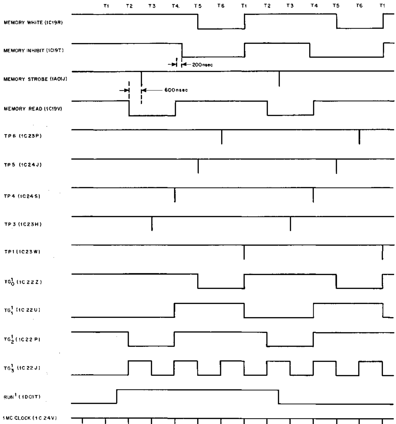
Figure 2-1 Timing Diagram
