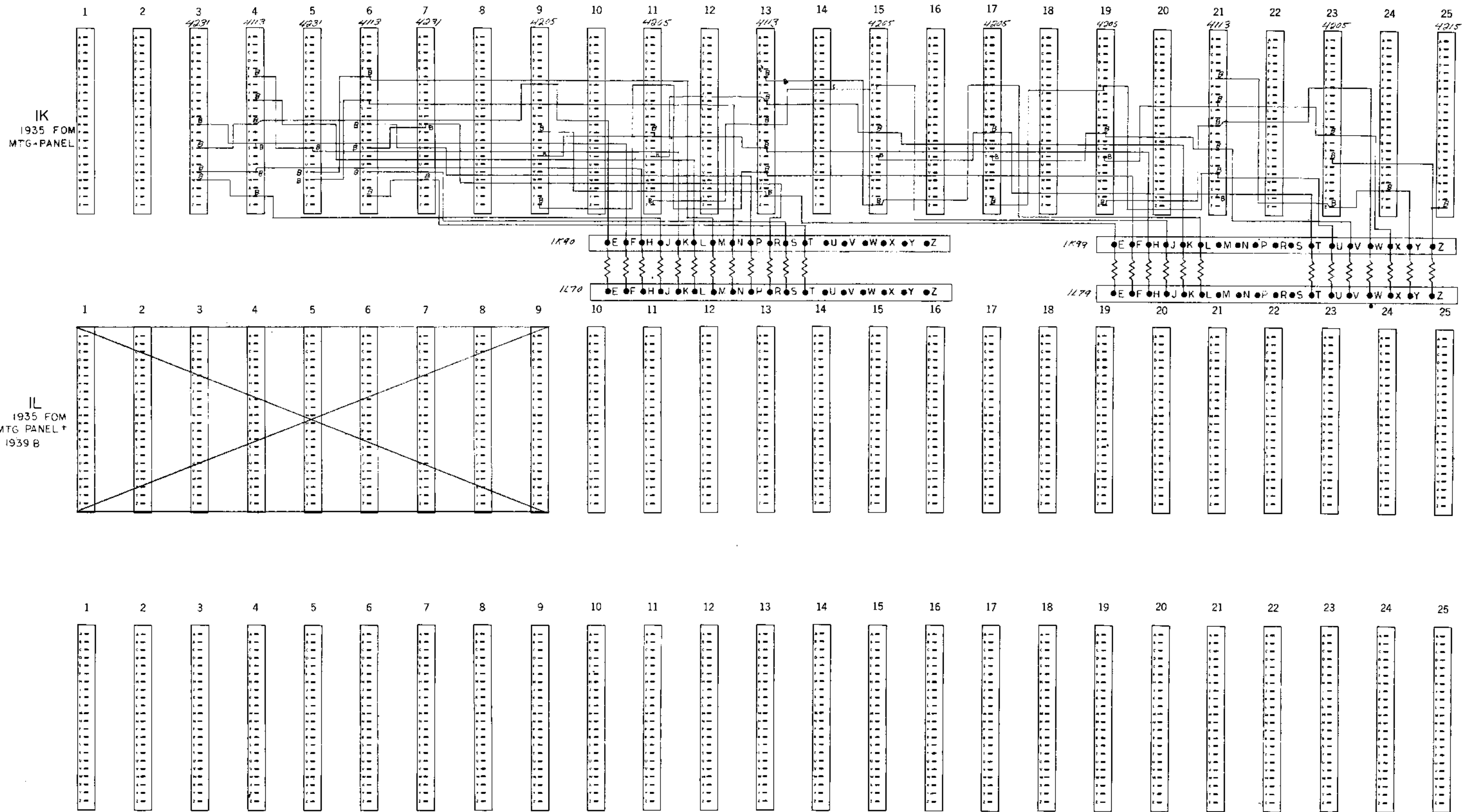
Wiring Diagram 1K and 1L (Sheet 1) WD-D-153-0-4
