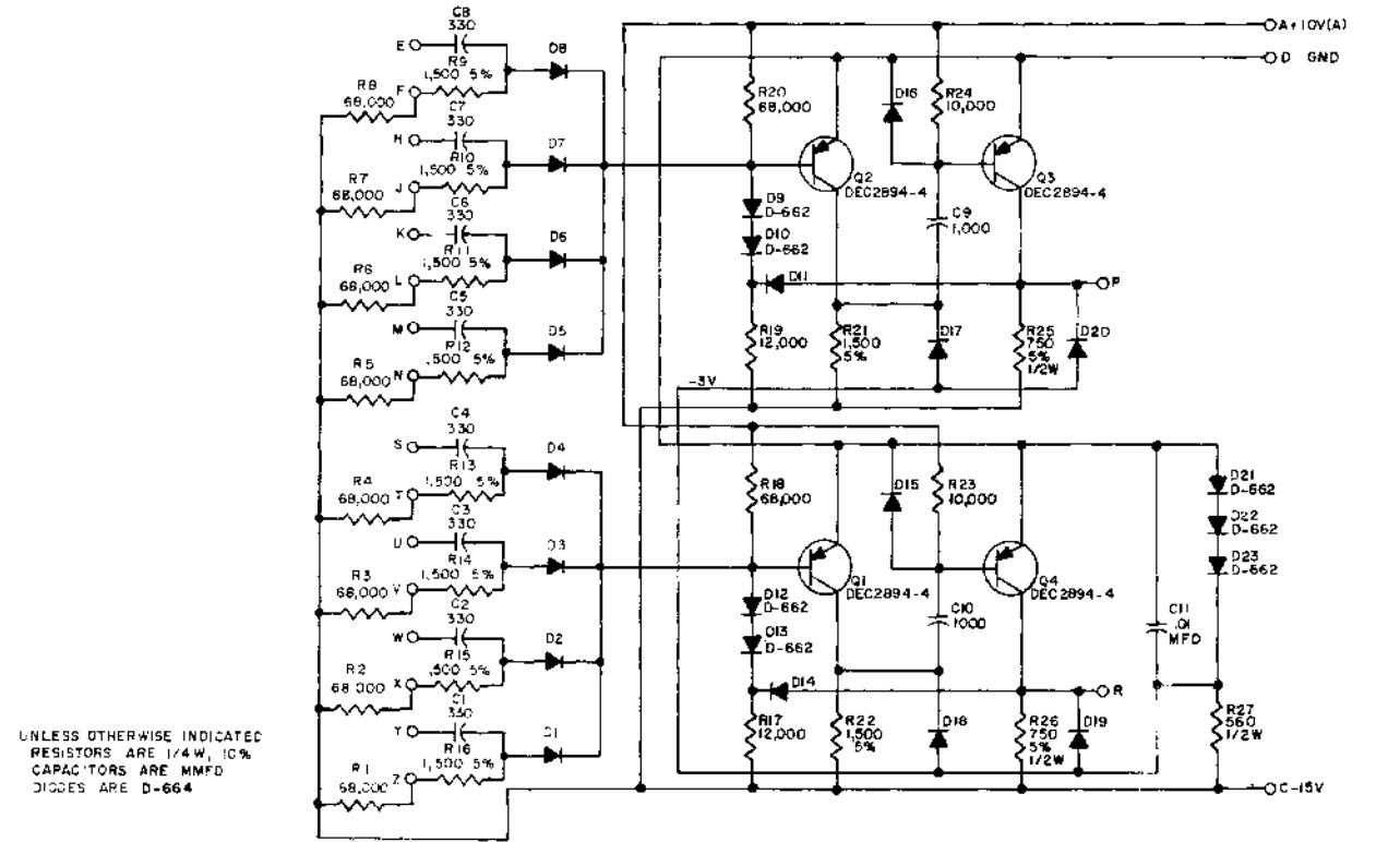
Positive Capacitor-Diode Gate RS-4130
