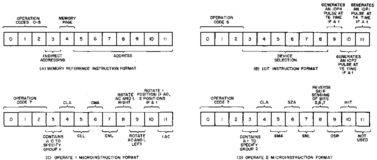
Figure 1-3 Instruction Formats
