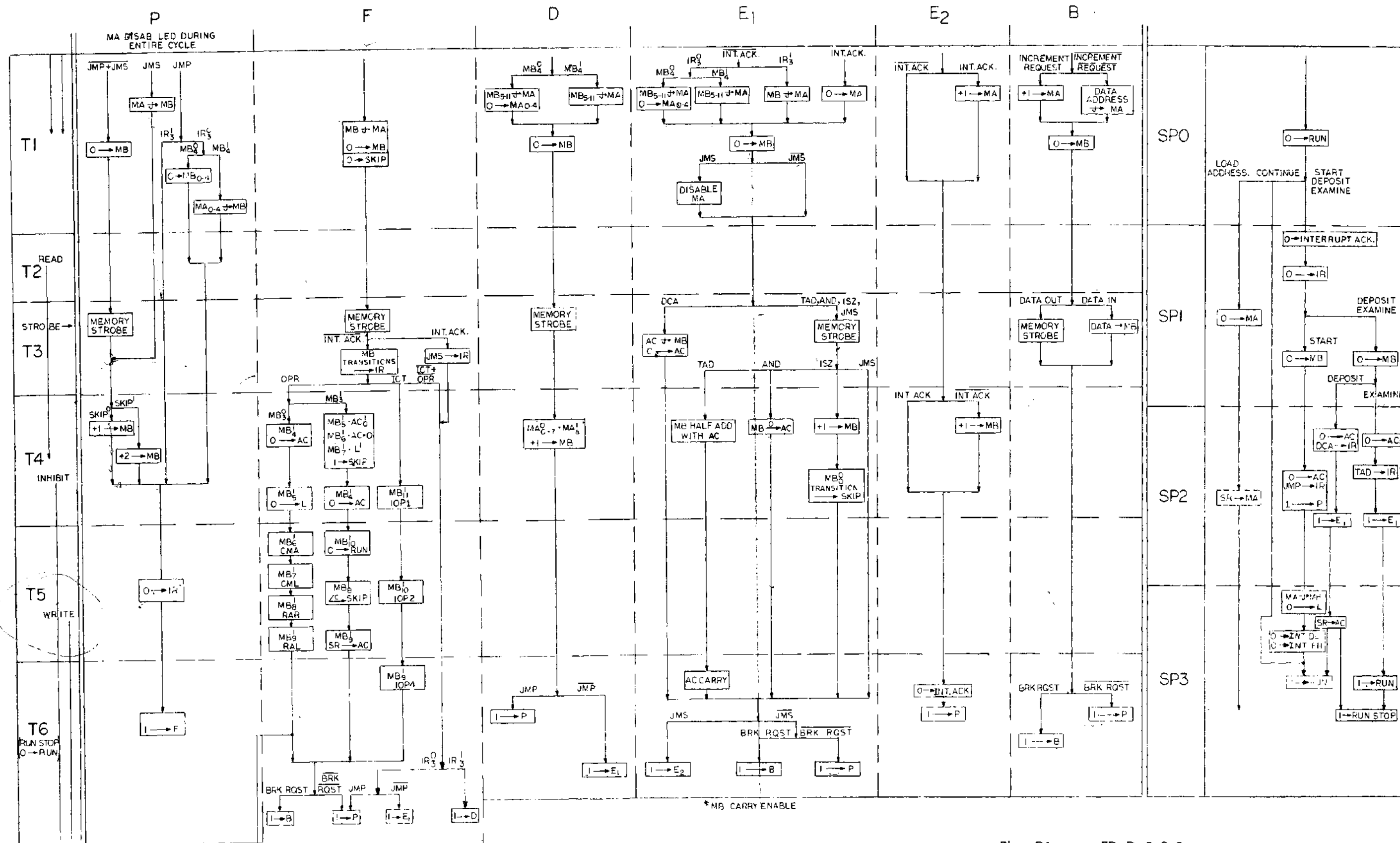
Flow Diagram FD-D-5-0-2
