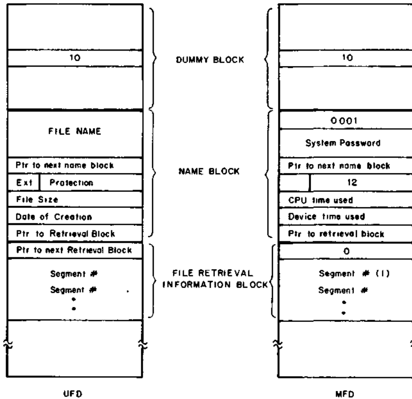
Figure 8-16 File Directories
