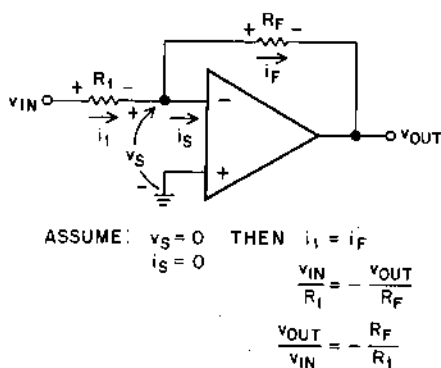
Fig. 2, Inverting Amplifier
