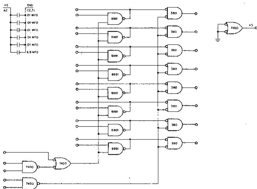
Figure 5 M785 Unibus Drivers and Receivers*
