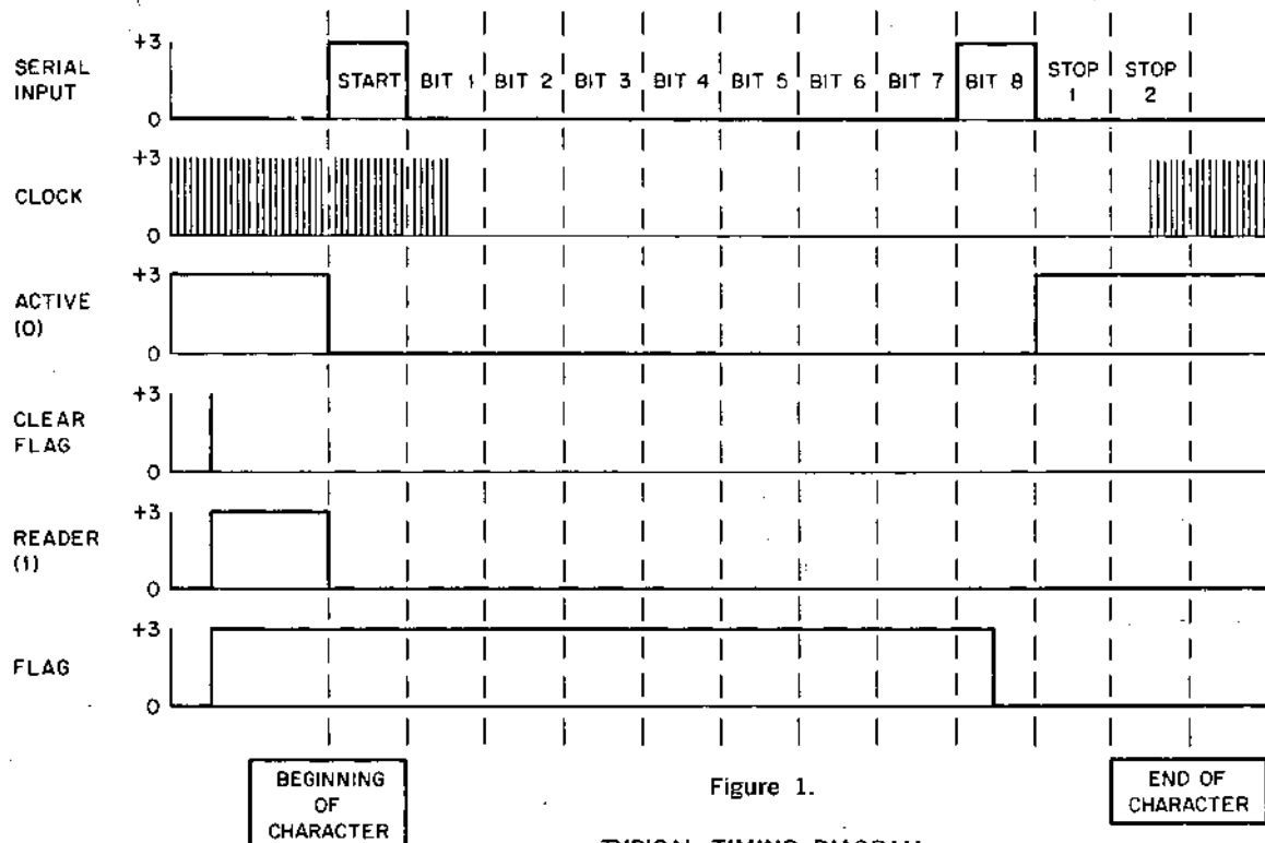
TYPICAL TIMING DIAGRAM
