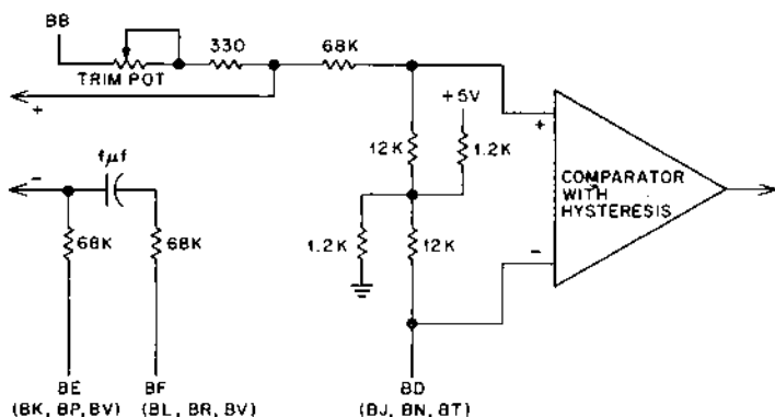
K524 EQUIVALENT CIRCUIT
