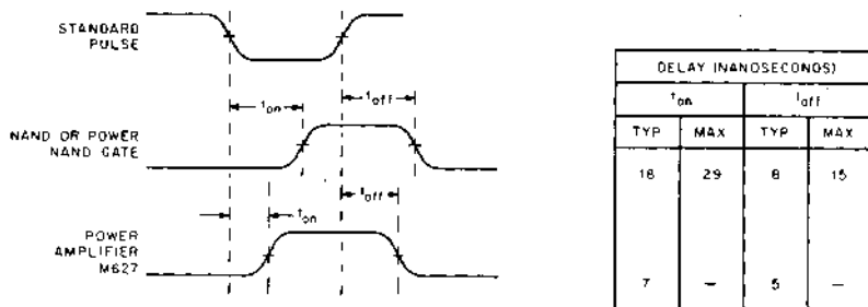
Figure 18. NAND Gate and Power Amplifier Delays
