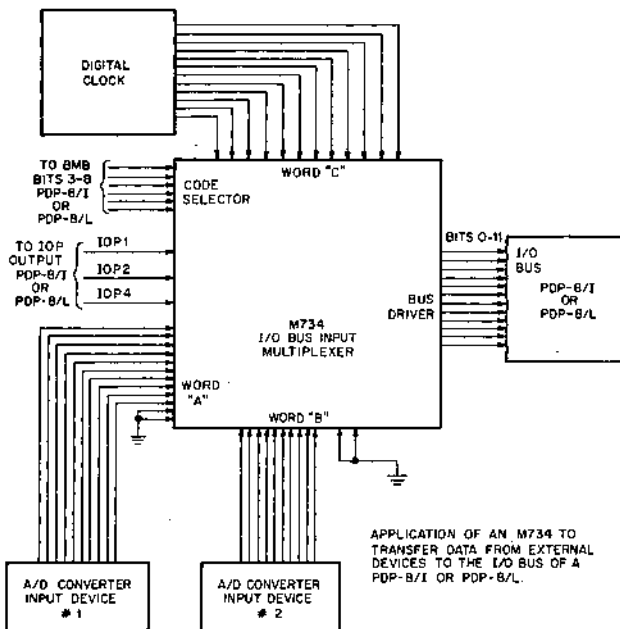
FIGURE 1. APPLICATIONS OF A M734 USED TO TRANSFER DATA FROM EXTERNAL DEVICES TO THE I/O BUS OF A PDP-8/L
