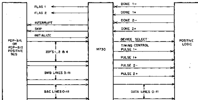
USE OF M730 ALONE
