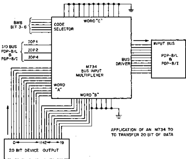
FIGURE 2. APPLICATION OF AN M734 TO TRANSFER 20 BIT OF DATA
