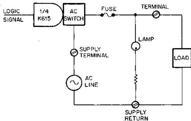
K615 CIRCUIT IN USE
