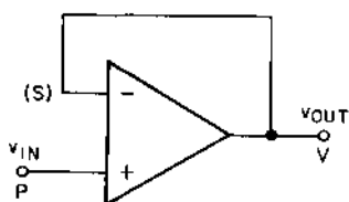
Fig. 5, Voltage Follower
