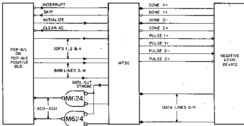
Figure 3. USE OF M732
