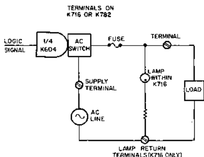
K604 CIRCUIT IN USE
