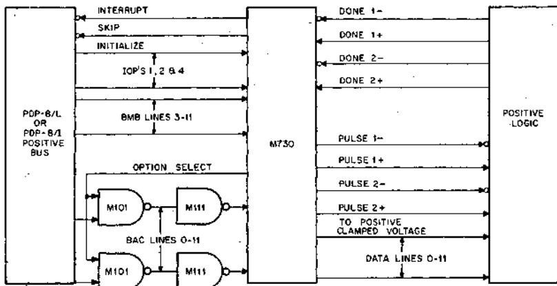
USE OF M730 USING M101 & M111
