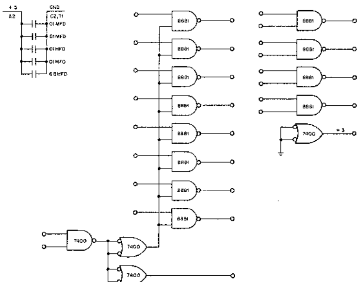
Figure 3 M783 Unibus Drivers*
