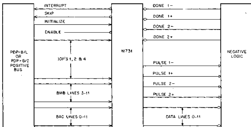
Figure 4. USE OF M731 ALONE
