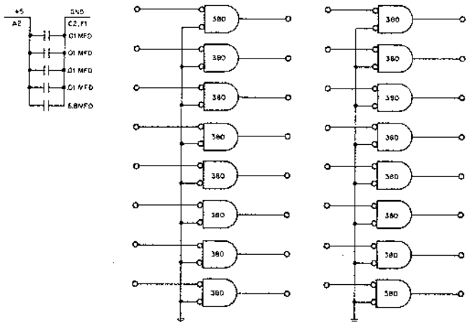
Figure 4 M784 Unibus Receivers*
