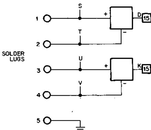
K522 SENSOR CONVERTER
