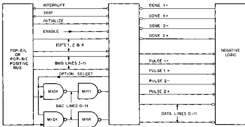
Figure 3. USE OF M731 USING M101 & M111
