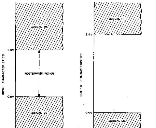
Figure 7 Logic Levels
