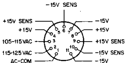
POWER SUPPLY 2
