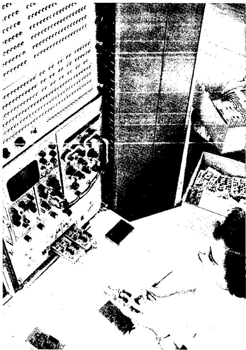
DEC thoroughly tests all finished modules, performing 100 ac and dc tests in less than 5 seconds. Most testing is done automatically on one of three computer-operated test stations like this one.
