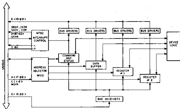
Figure 1. Typical Peripheral Device Interface
