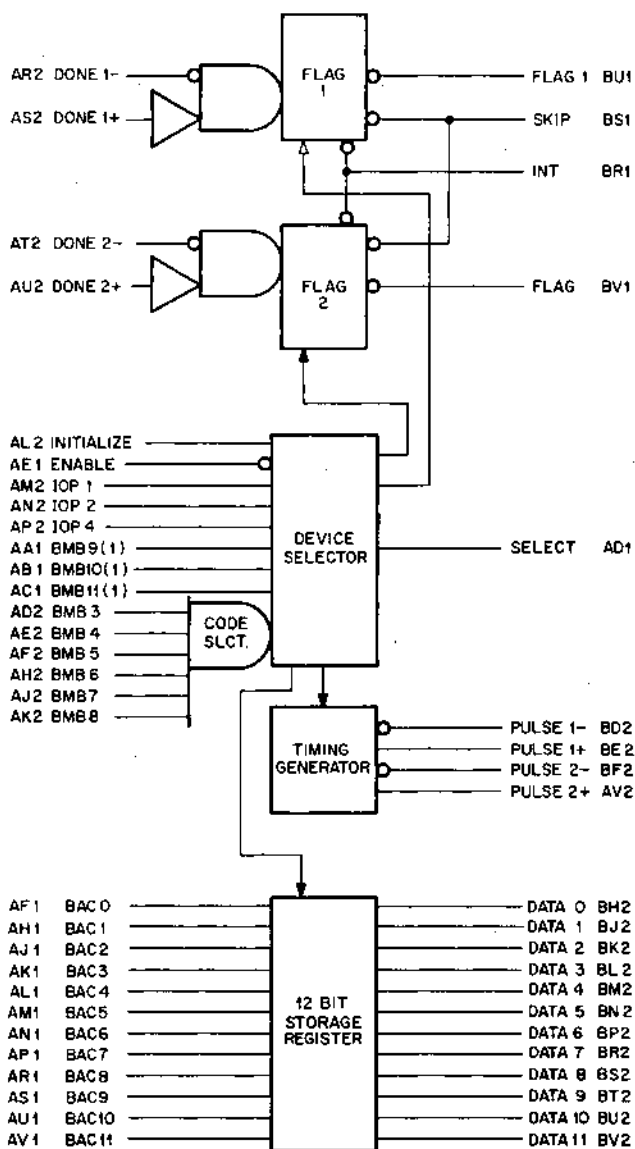
M730 POSITIVE OUTPUT INTERFACE FOR POSITIVE BUS 8/I OR 8/L
