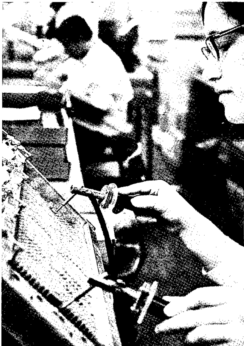
This subassembly process depicts the soldering of bussing strips. A high current passes through the bus strip to evenly distribute all solder.
