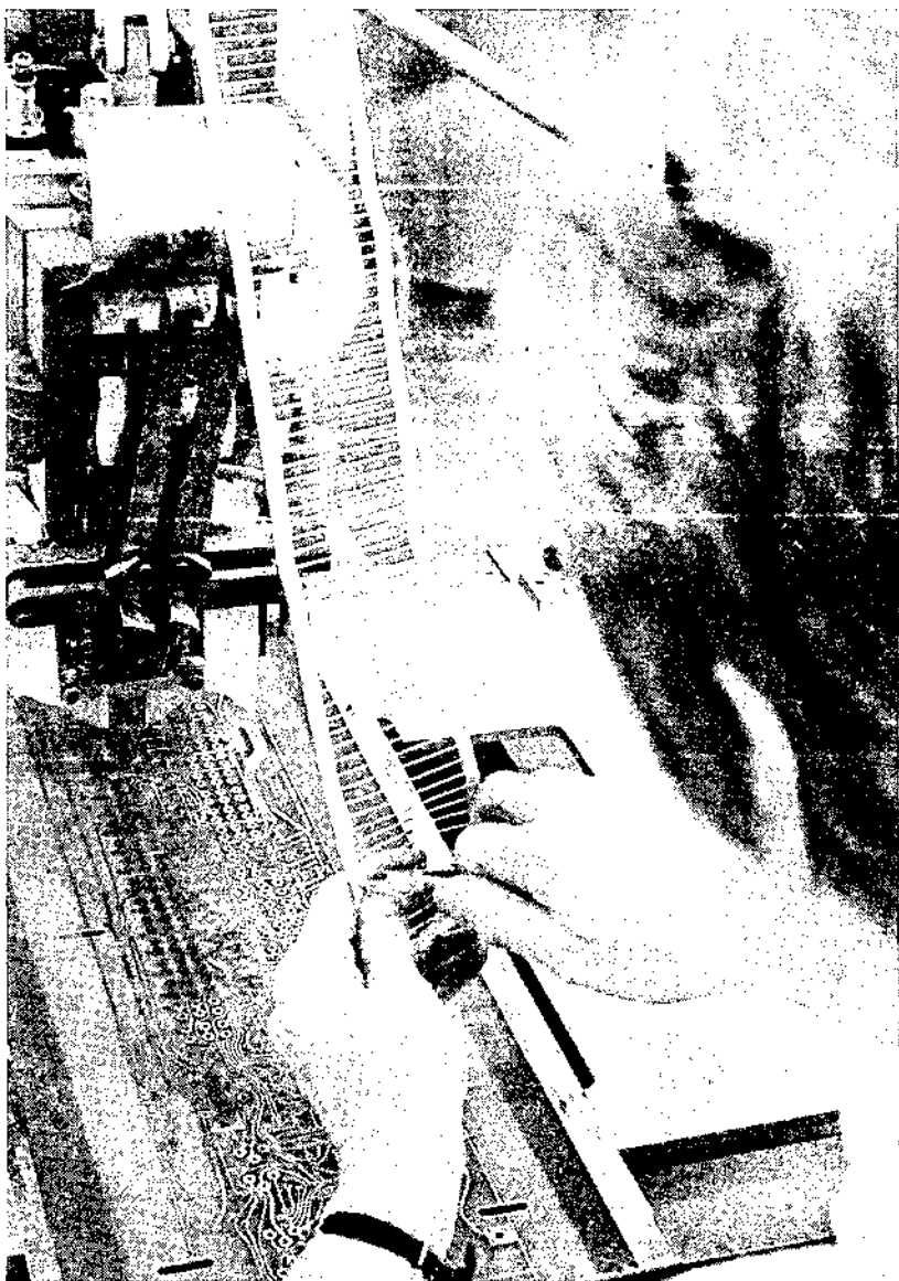
These pantograph-controlled insertion machines position and crimp pre-tested components onto four module boards at a time. A press will cut the modules apart after assembly is completed, minimizing handling up to that point.
