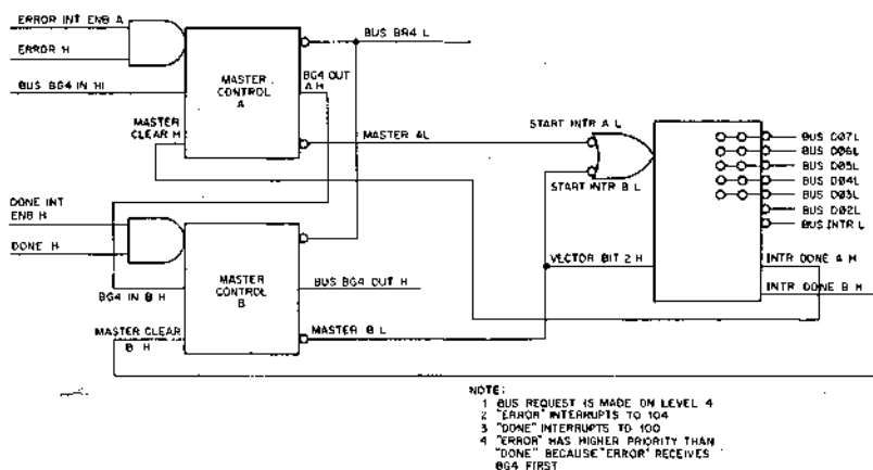
Figure 9. Typical Interconnection of M782 Interrupt Control
