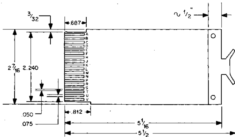
SINGLE-HEIGHT FLIP CHIP MODULE
