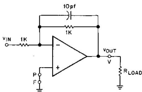
Fig. 6, Inverter
