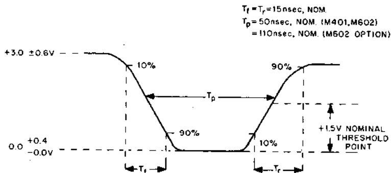
Figure 17. Standard Pulse
