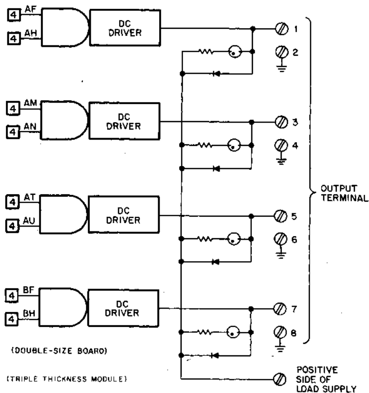
K658 4 AMP DRIVER
