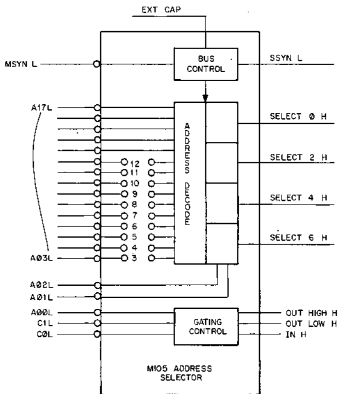
Figure 6 M105 Address Selector
