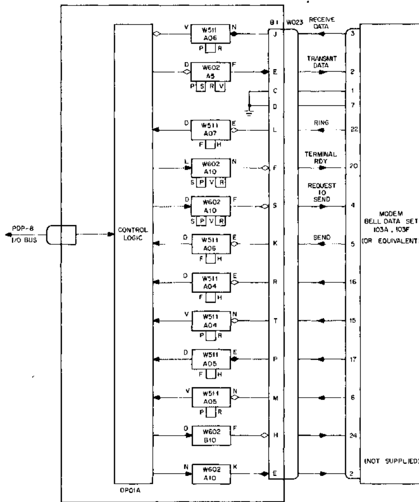
Figure 3-19 DP01A Data Set Interface
