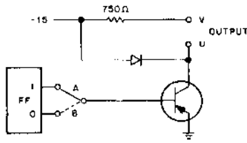
Figure 3-9 W750 Output Circuit Simplified Schematic
