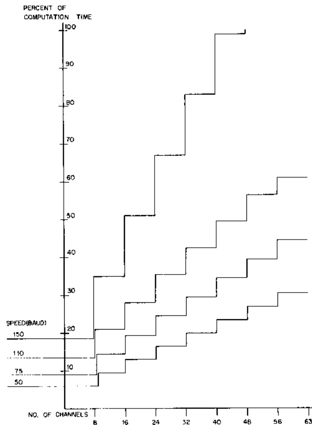
Figure 3-6 680 Processor Loading
