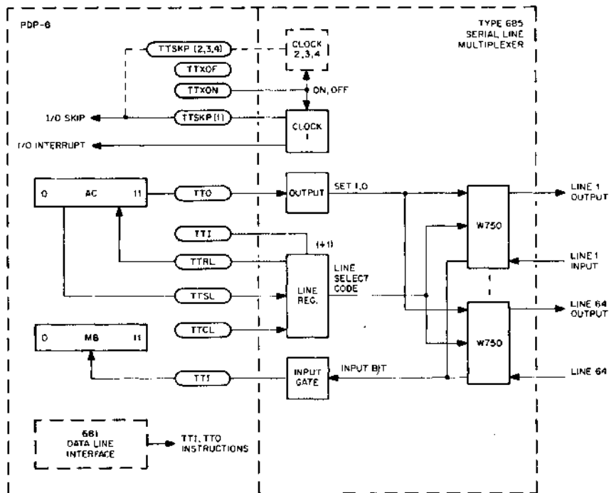
Figure 3-5 680 System Functional Block Diagram
