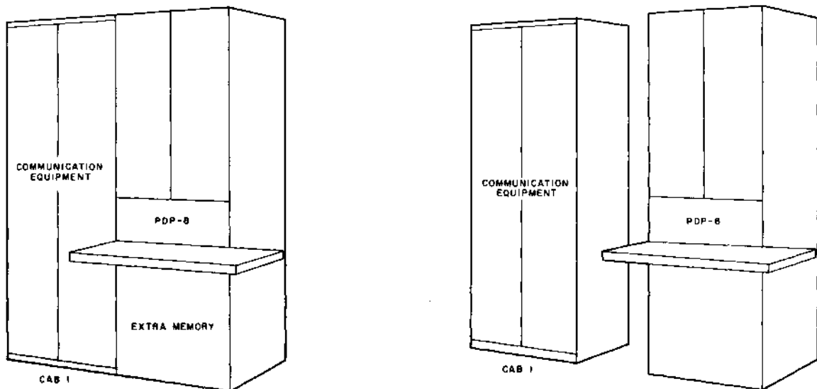
Figure 3-16 680 Communication System Cabinet Arrangement
