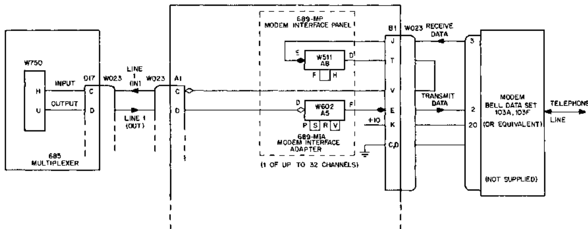
Figure 3-14 689-MP and 689-MIA Modem Interface
