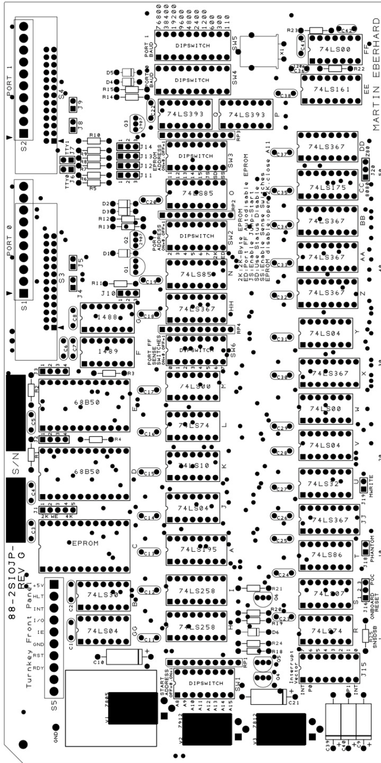
Rev G PC Board Component Placement
