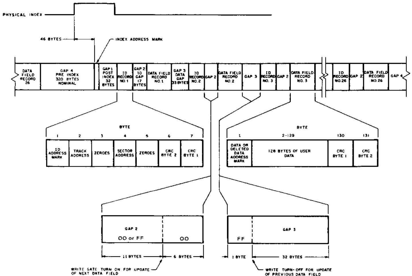
FIG.13 TRACK FORMAT
