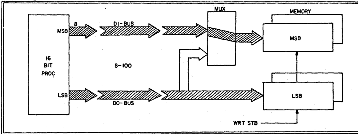
FIGURE 3 16 BIT WRITE
