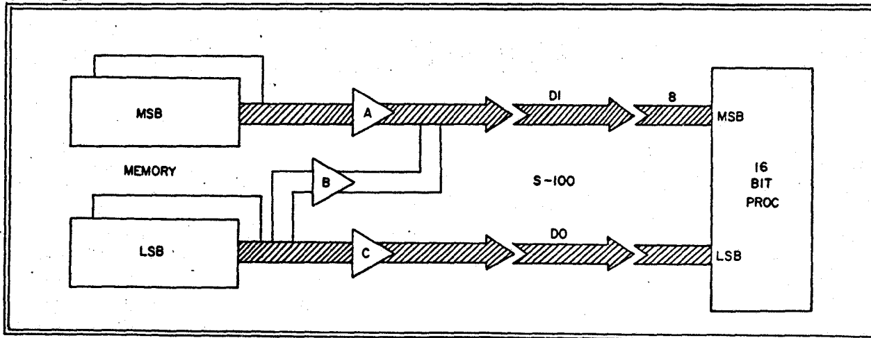
FIGURE 4 16 BIT READ
