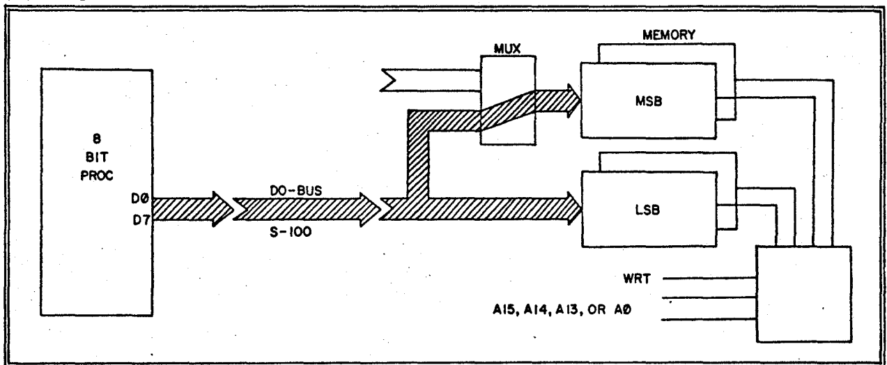
FIGURE 5 8 BIT WRITE
