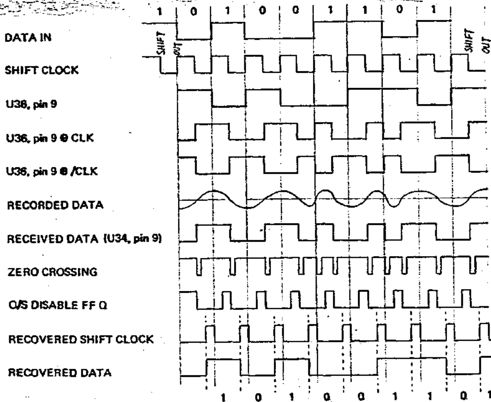
Figure 1 Timing Diagram
