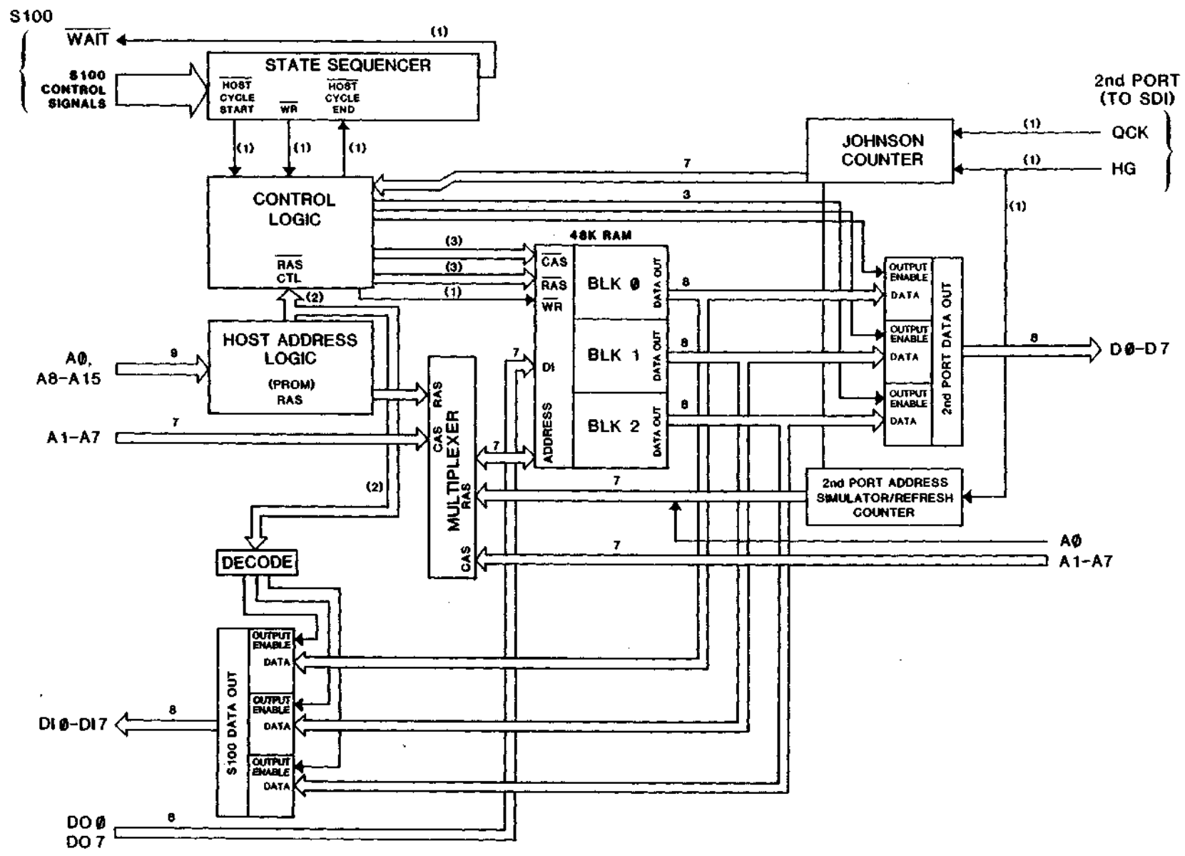
Figure 12 - 48KTP Block Diagram
