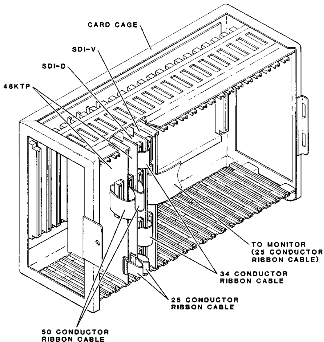
Figure 6 - SDI and 48KTPs in Card Cage
