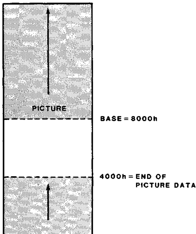
Figure 8 - "Wrap Around" Base Address
