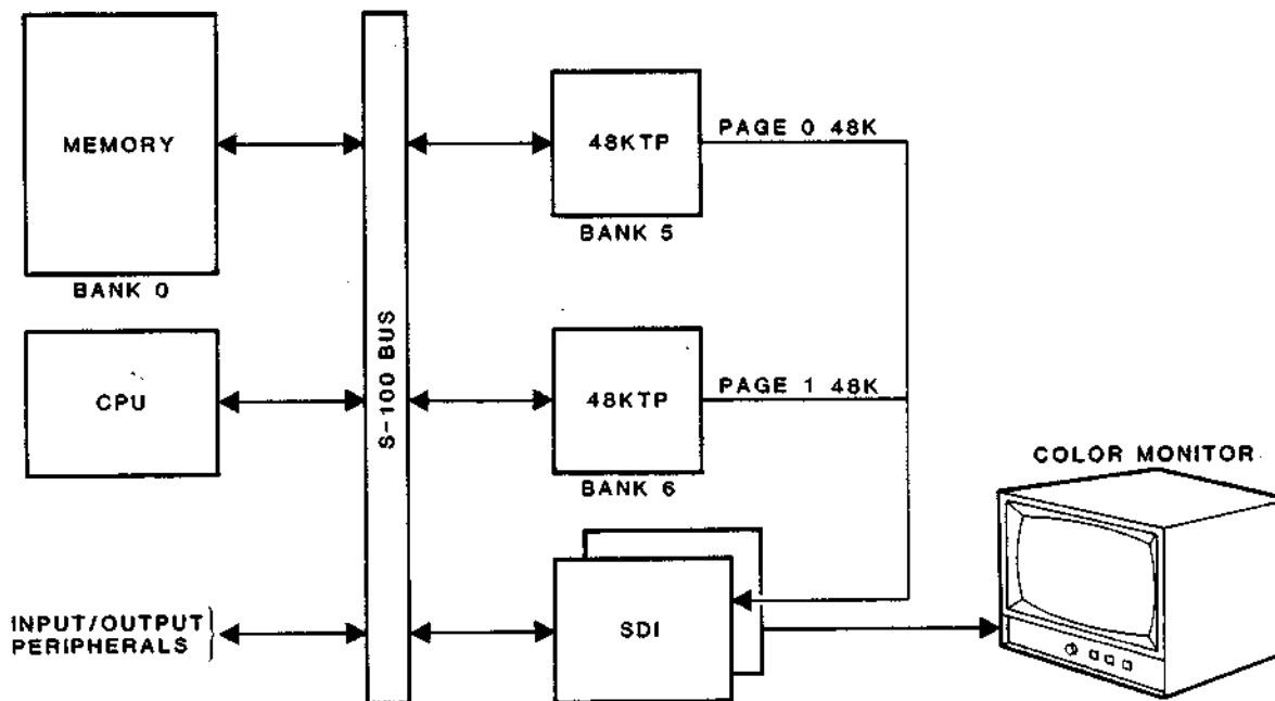
Figure 2 - An SDI System with Two 48KTP Boards
