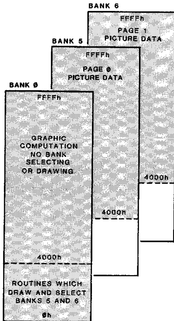
Figure 5 - Organization of the SDI and 48KTP
