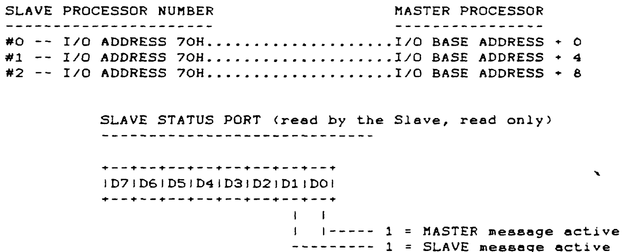
Figure 2-5 Slave Status Port Bit Definitions
