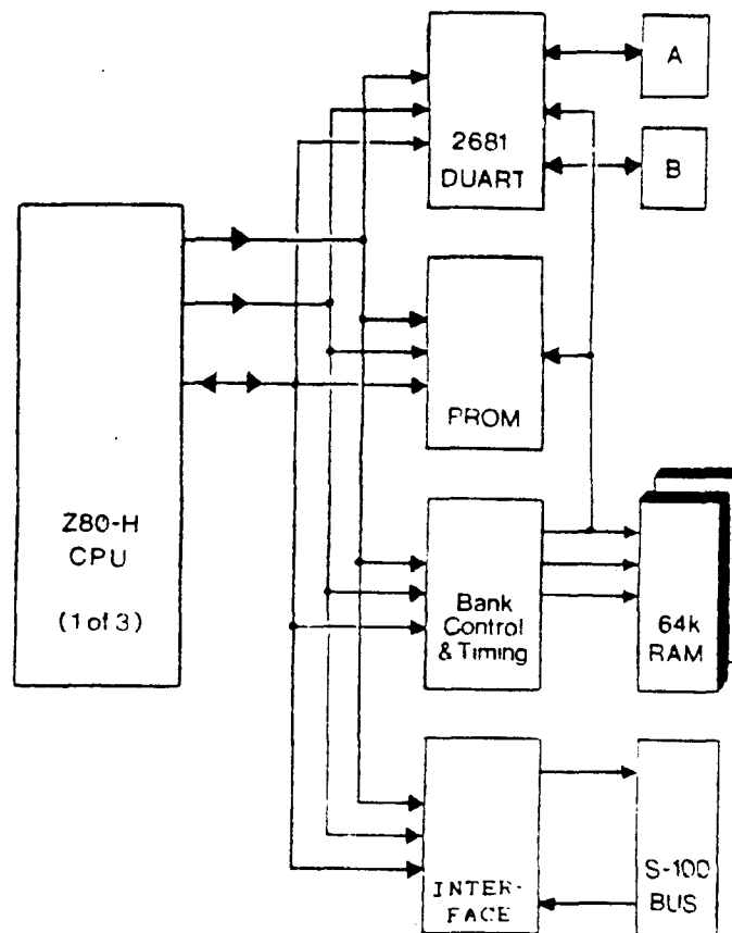
Figure 1-1 Multi Slave Block Diagram
