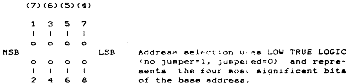
Figure 2-3 Multi Slave Base Address Selection
