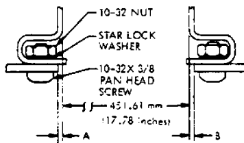
Figure 2-9. Inside Measurement Between Slide Brackets
