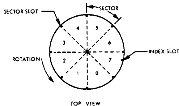
Figure 1-5. Mechanical Sectoring
