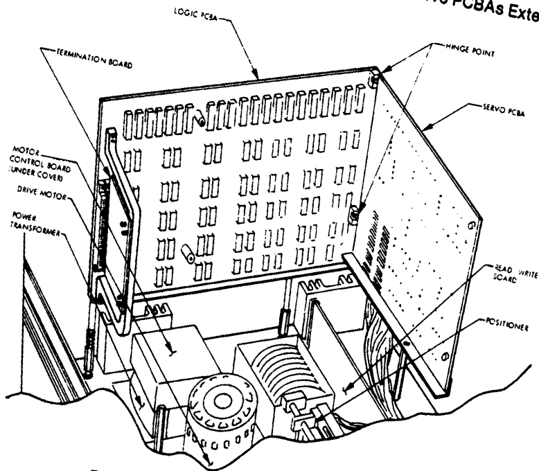
Figure 2-4. Component Identification
