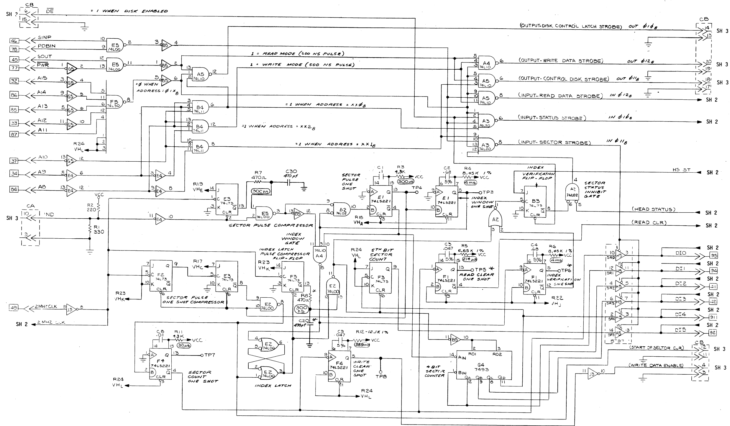
MITS 3200 SCHEMATIC DIAGRAMS DISK BOARD #1 (Sheet 1 of 3) ADDRESS/I-O SELECT & SECTOR CIRCUITS
