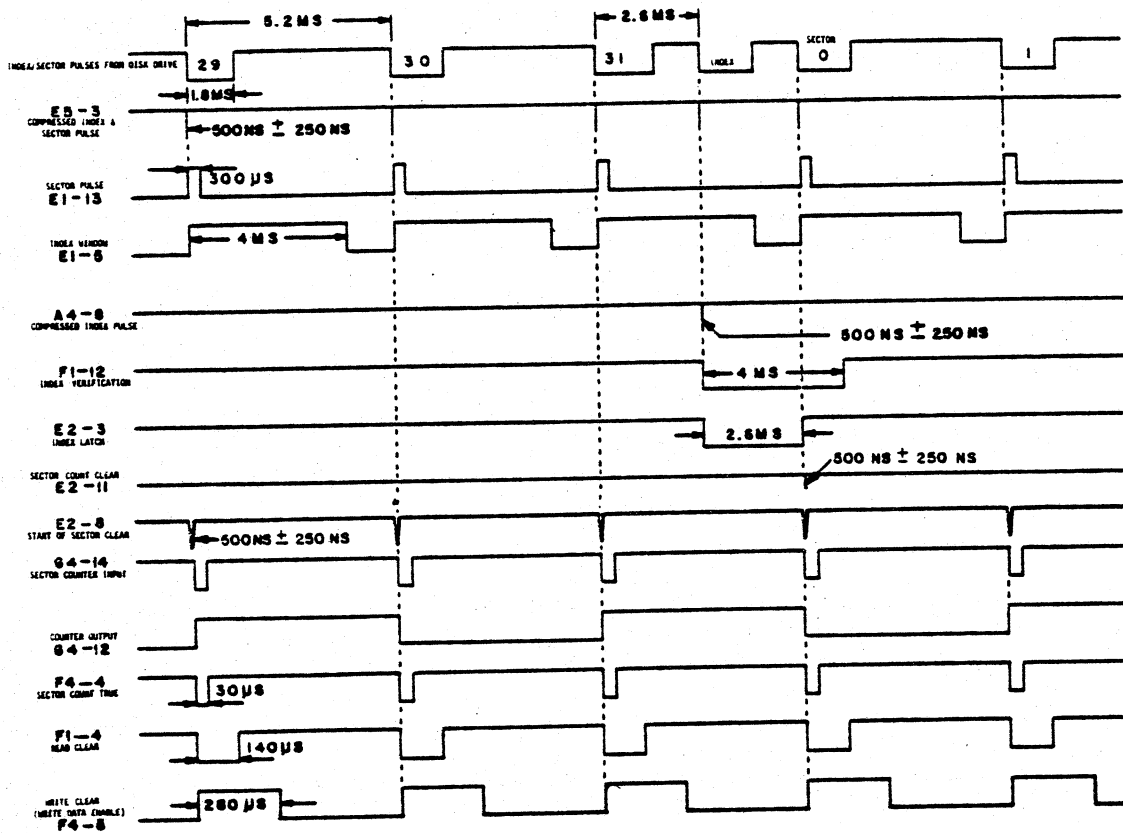
Index/Sector Timing
