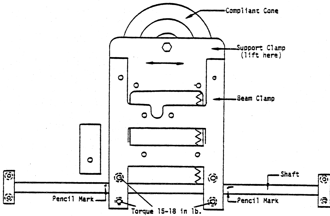
Cone Clamping Mechanism Adjustment
