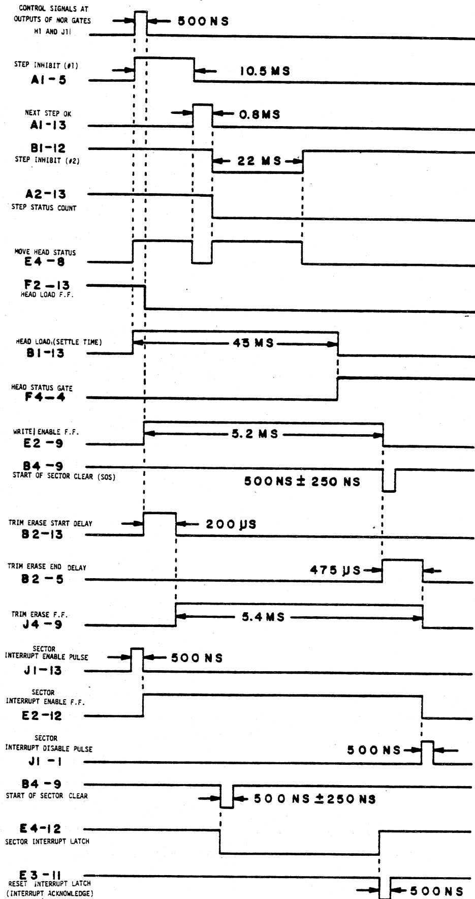
Disk Function Control Timing Diagram
