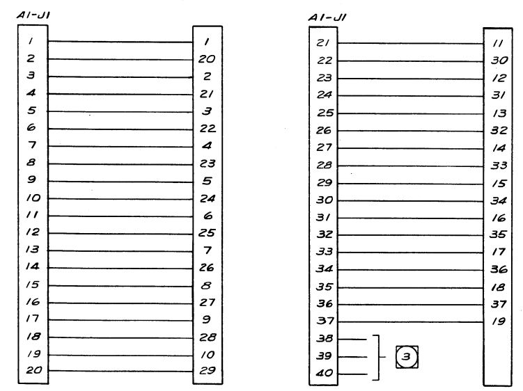
WIRING DIAGRAM
