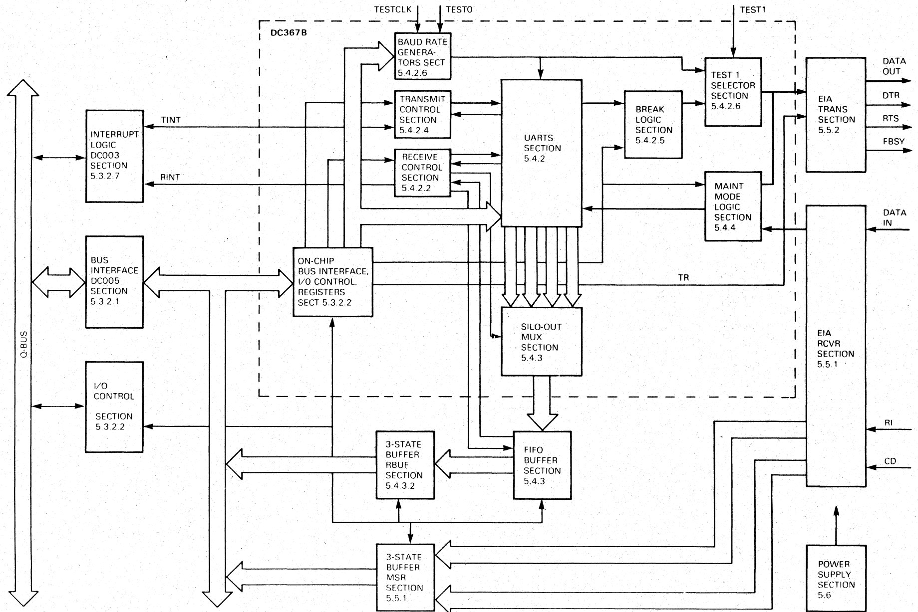
Figure 5-2 Simplified Functional Block Diagram
