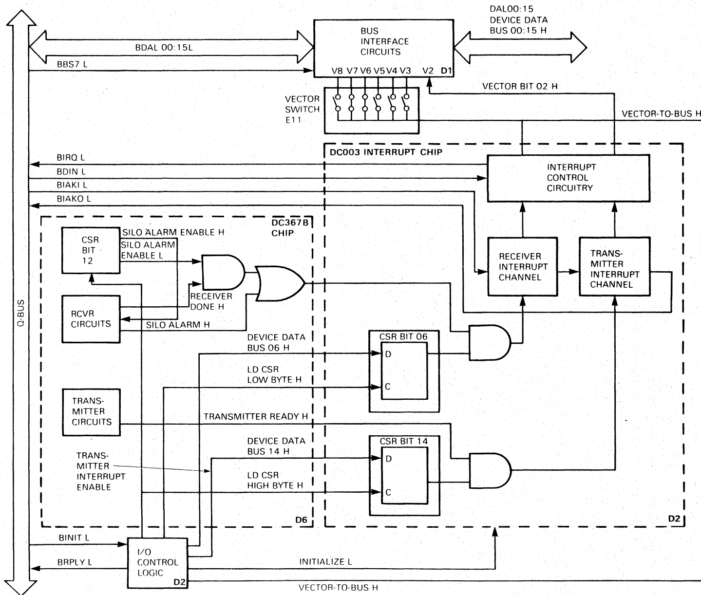
Figure 5-7 Interrupt Logic
