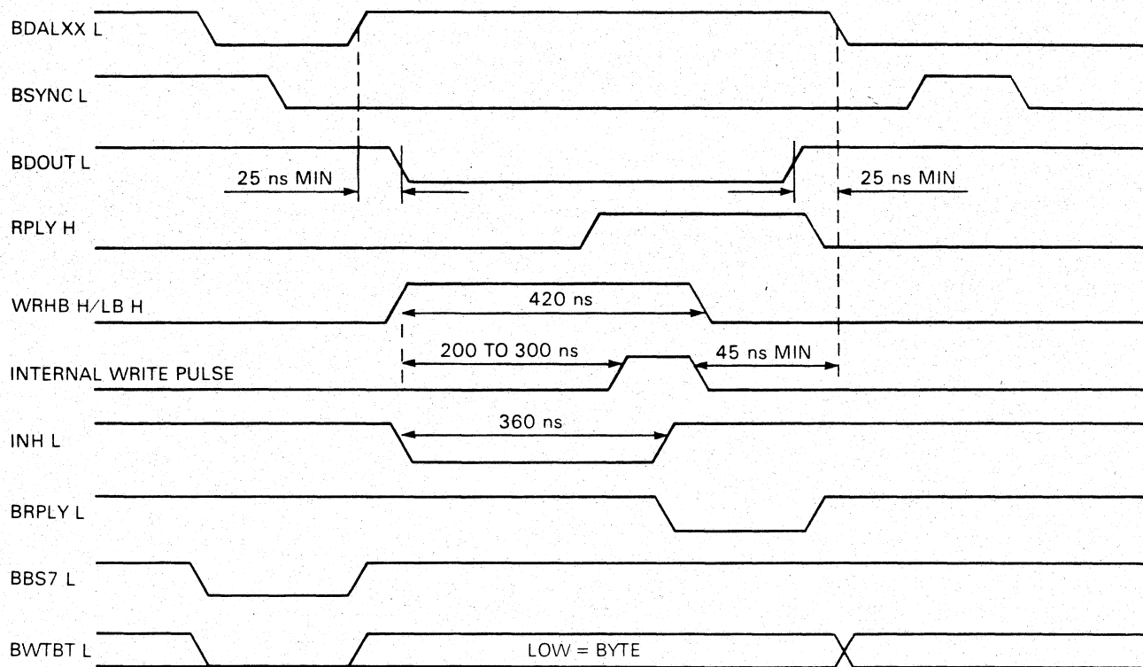
Figure 5-5 Data Output Timing
