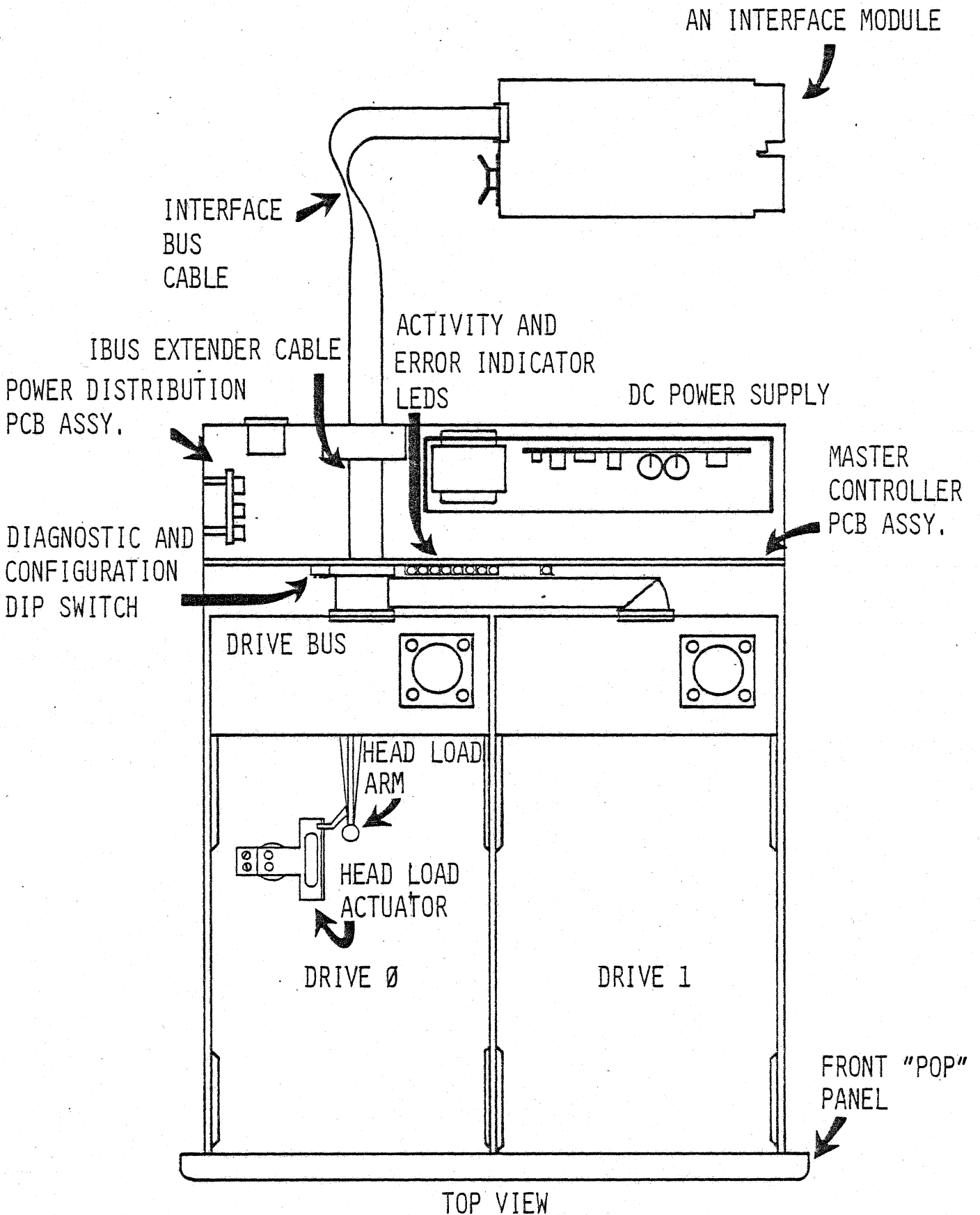
FIGURE 2-1 THE DSD 440 SYSTEM
