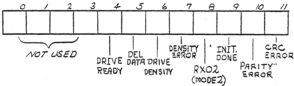
FIGURE 5-17 ERROR/STATUS REGISTER IN MODE 2
