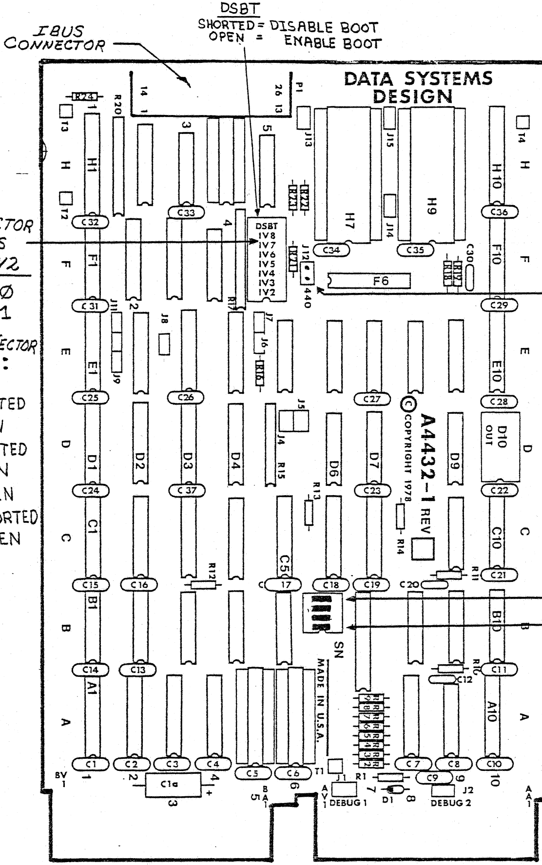
FIGURE 3-4 LSI-11 INTERFACE MODULE
