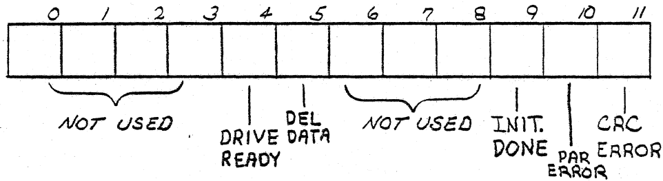
FIGURE 5-16 ERROR/STATUS REGISTER IN MODE 1
