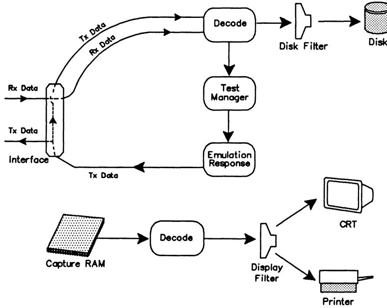
Figure 10-3 BSC Emulation Data Flow Diagram - Freeze Mode
