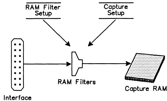
Figure 4-1 BSC Data Flow Diagram – Capture to RAM
