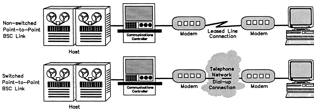
Figure A-1 Point-to-Point Configuration
