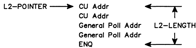
Figure C-1 General Poll Sequence
