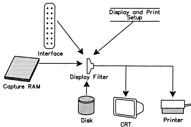
Figure 6-1 BSC Data Flow Diagram – Display and Print
