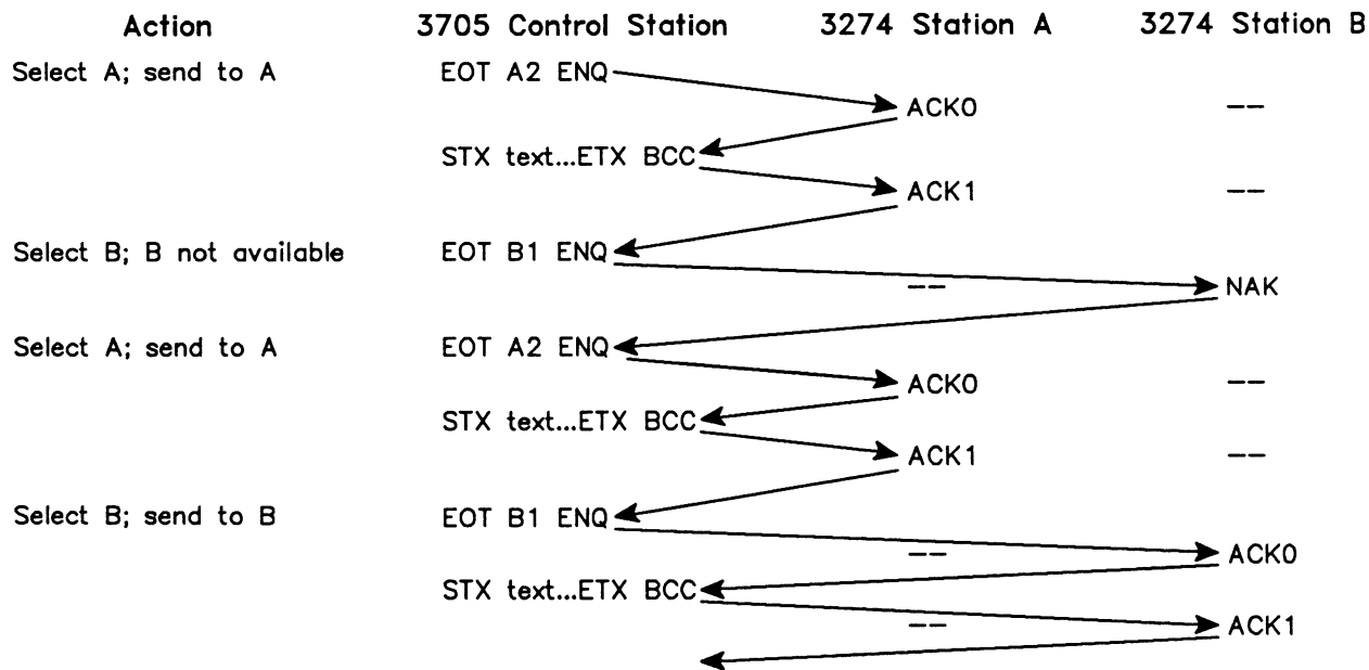
Figure A-5 Multipoint Select Sequence Transmission
