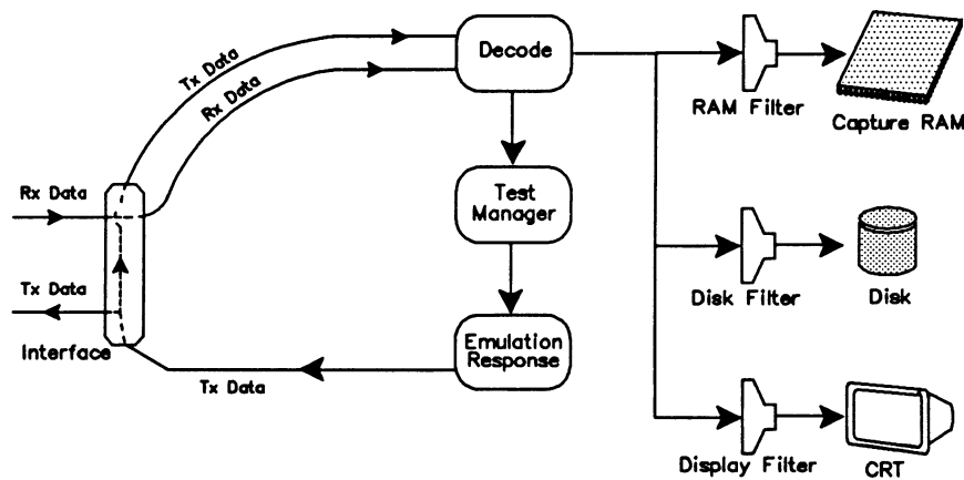
Figure 10-1 BSC Emulation Data Flow Diagram - Live Data
