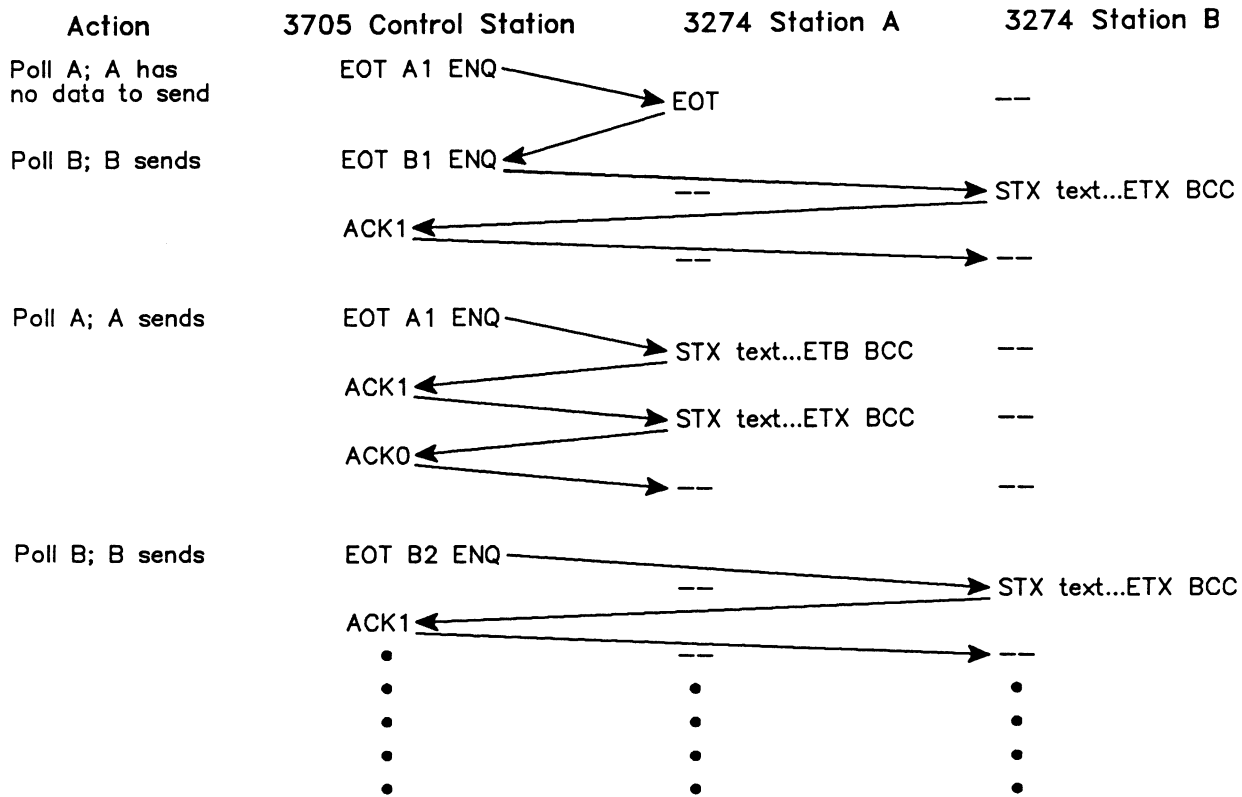
Figure A-4 Multipoint Polling Sequence Transmission
