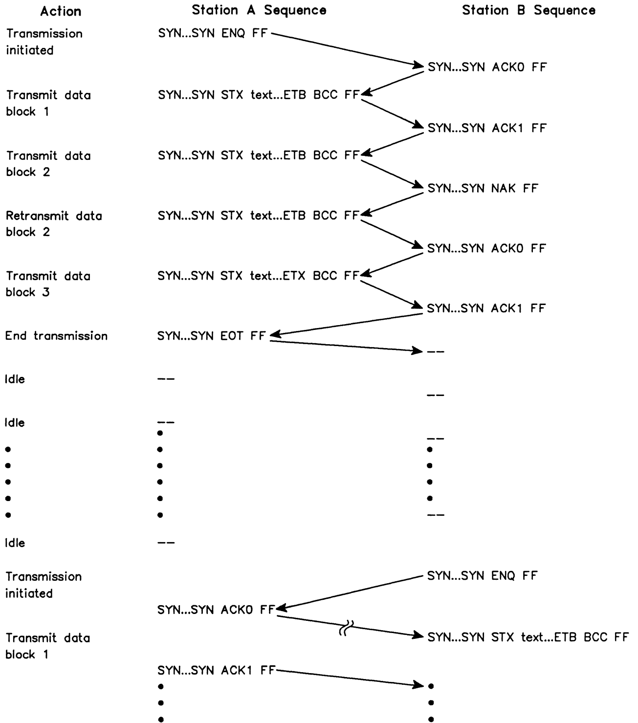
Figure A-3 Point-to-Point Setup and Transmission
