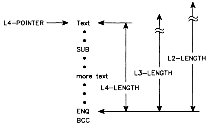
Figure C-5 Test Request Message
