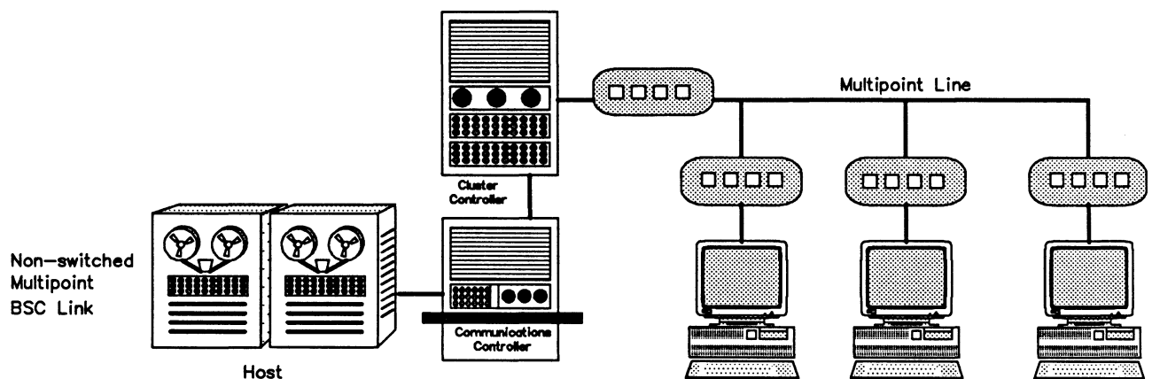
Figure A-2 Multipoint Configuration
