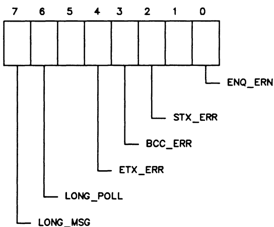
Figure 11-1 ERROR-GEN Bit Position
