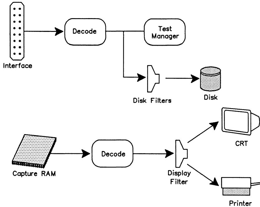
Figure 3-3 BSC Monitor Data Flow Diagram - Freeze Mode
