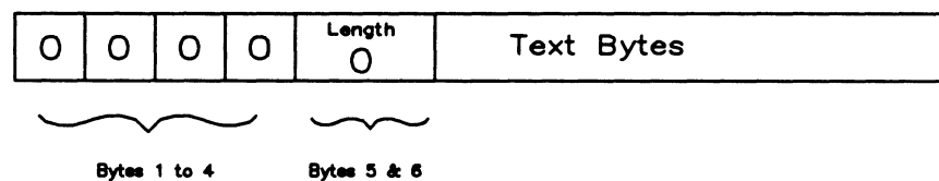
Figure 12-1 Buffer Structure
