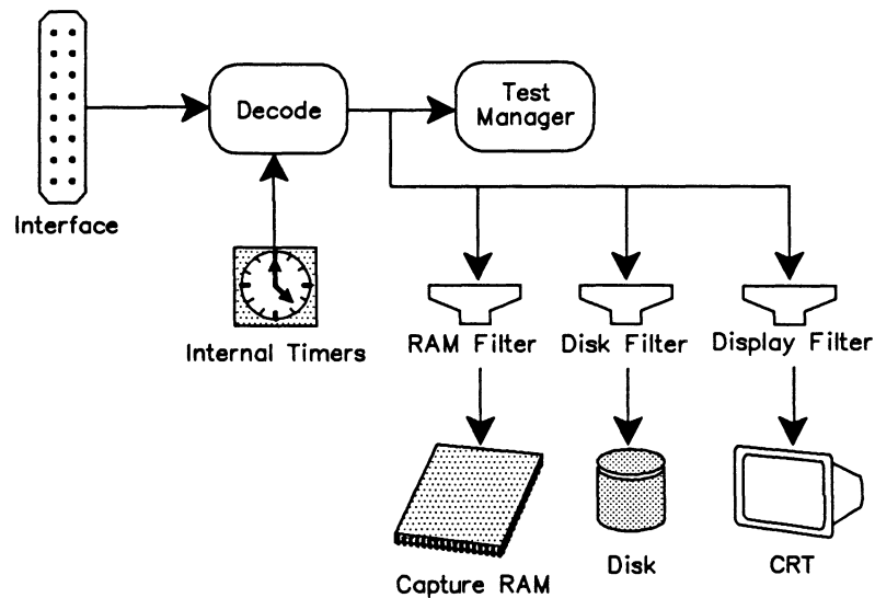
Figure 3-1 BSC Monitor Data Flow Diagram – Live Data
