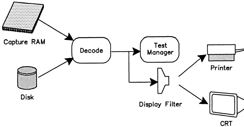
Figure 3-2 BSC Monitor Data Flow Diagram – Offline Processing
