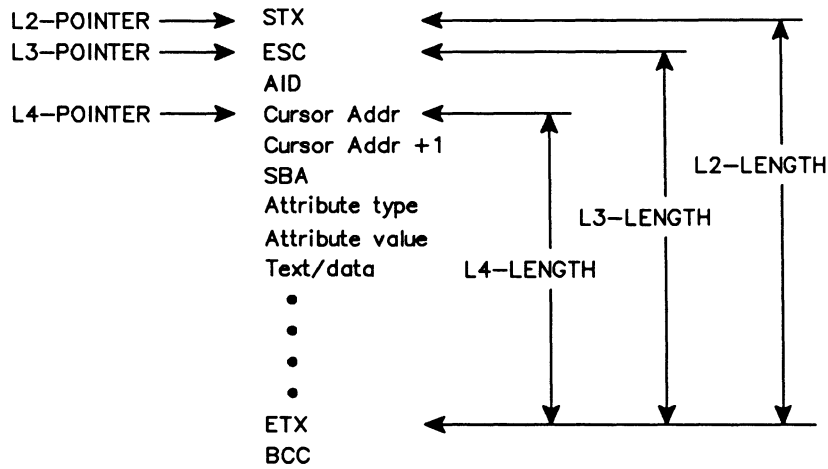
Figure C-9 Read Buffer Command
