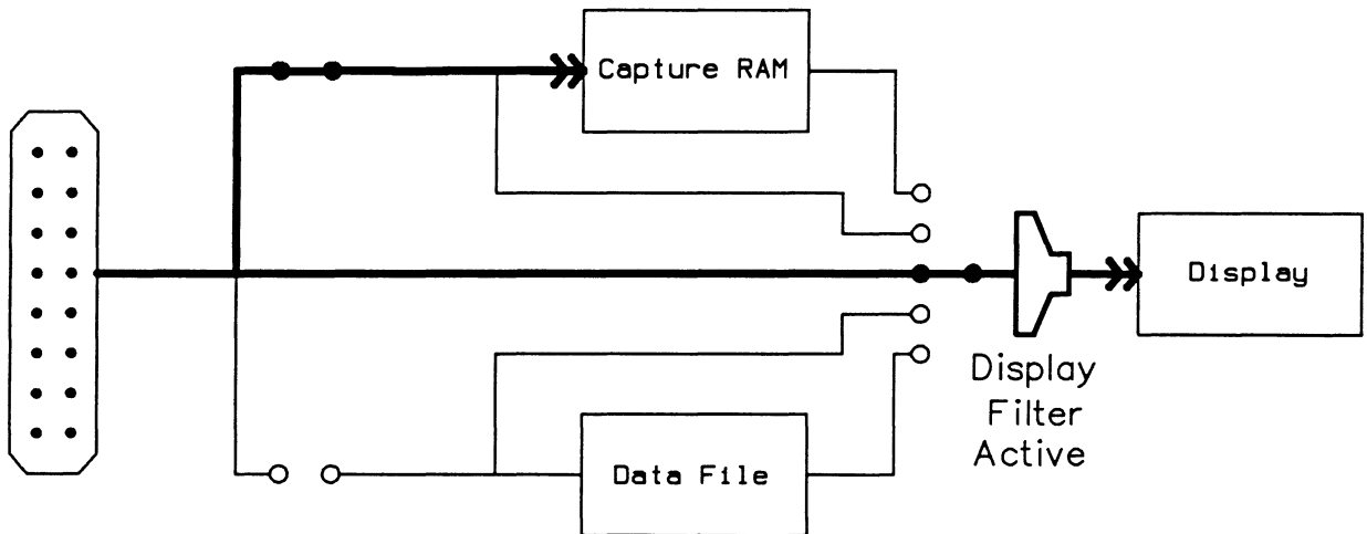
Figure 7-2 Connection Diagram - Display Filters Activated
