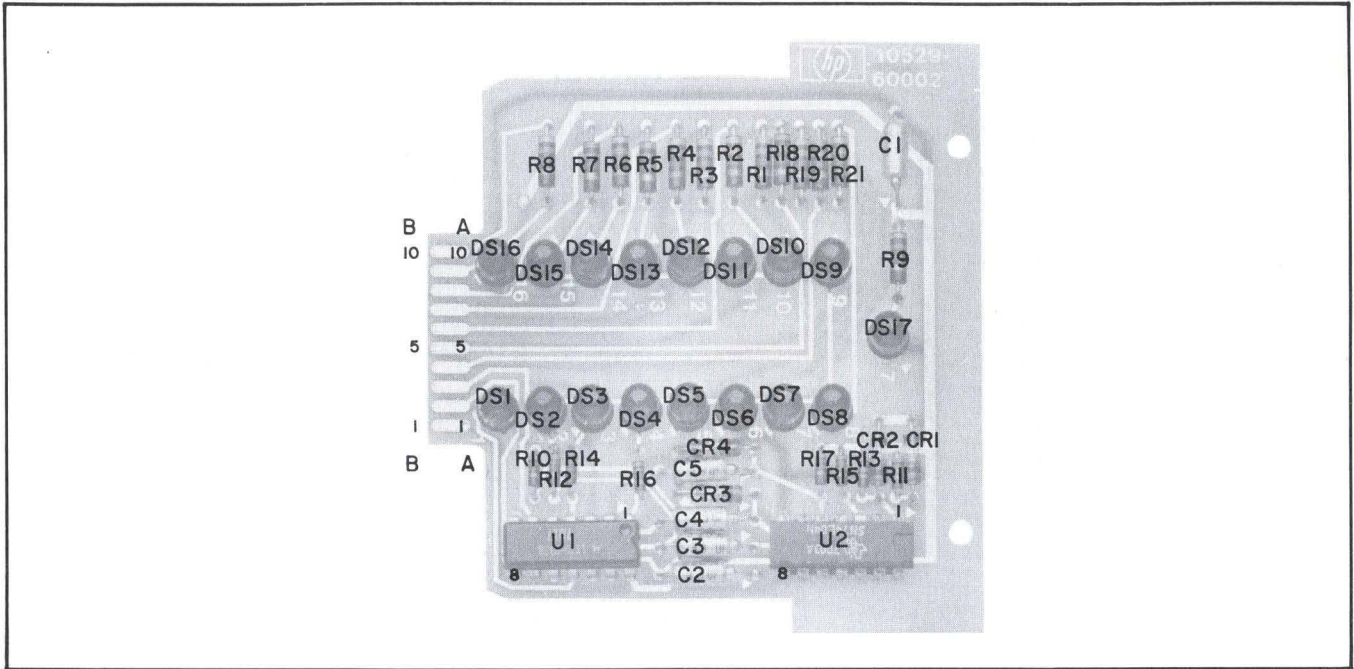
Figure 8-4. Display Board Component Locations
