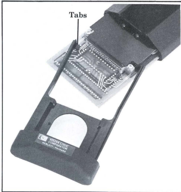
Figure 5-3. Removing Drawer
