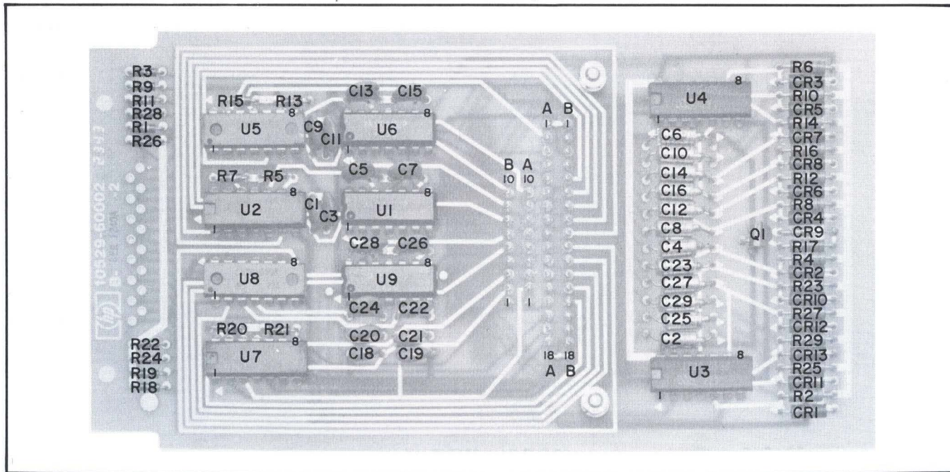
Figure 8-3. Main Board Component Locations
