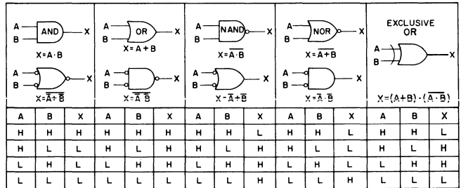
Figure 4-1. Gate Symbols and Logic Comparisons
