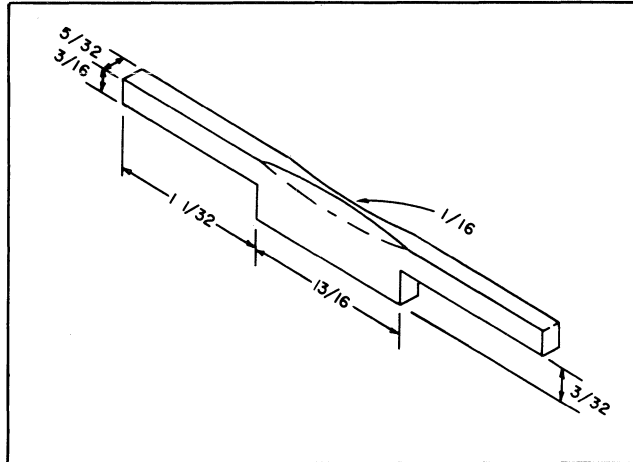
Figure 5-6. Extractor Tool
