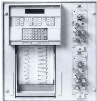
Gould Portable Two-Channel RS3200 Recorder (Model 30-V7202-10)
