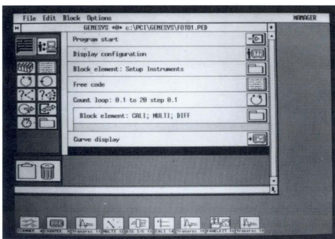
An icon-based program generator for IEEE-488 instrument control
