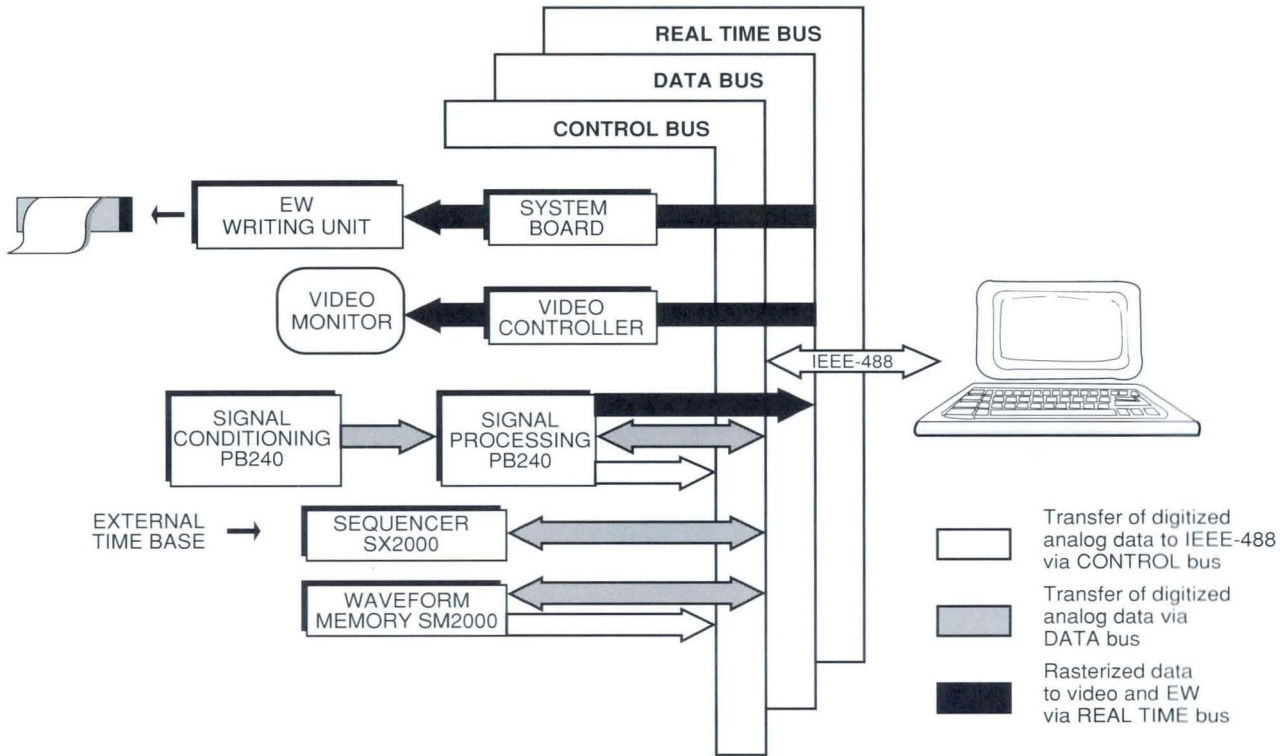
ES2000 Waveform Recording and Real Time Display System diagram
