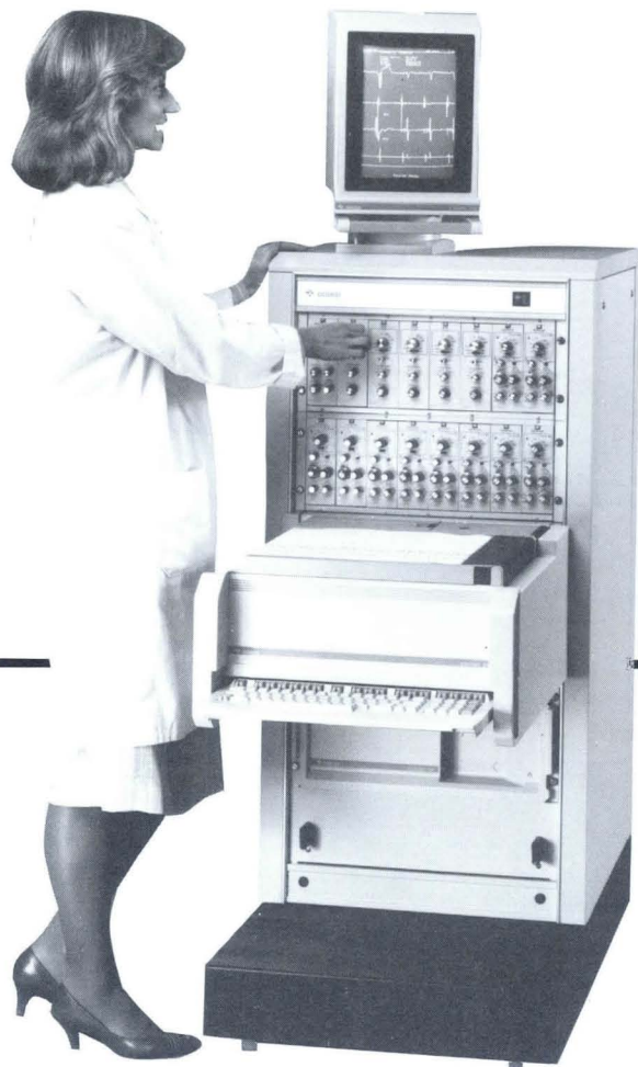
Gould ES2000 Medical Research Recording System
