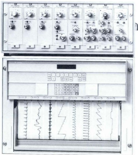
Gould Benchtop Eight-Channel RS3800 Recorder (Model 30-V7808-12). Configuration for benchtop six-channel RS3600 Recorder is the same, with amplifiers on top.
