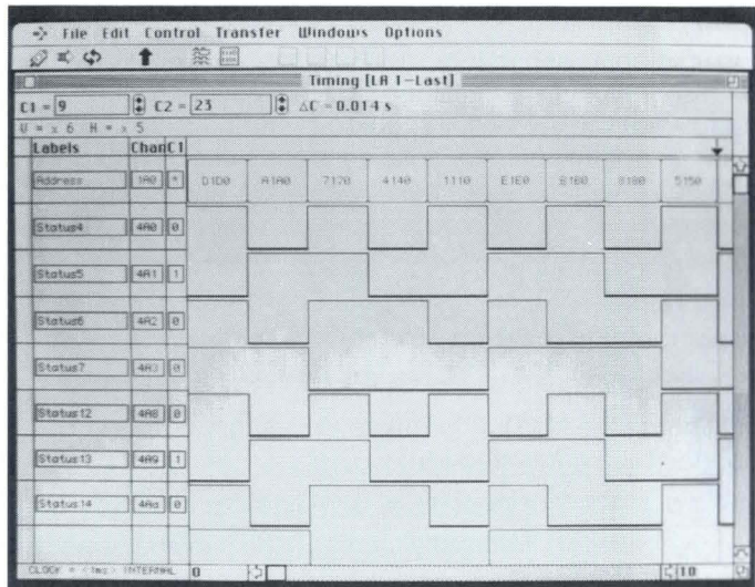
Timing: Displays timing waveforms for individual signals or buses. Two cursors measure time or cycles. Cursors also move through the State listing simultaneously.
