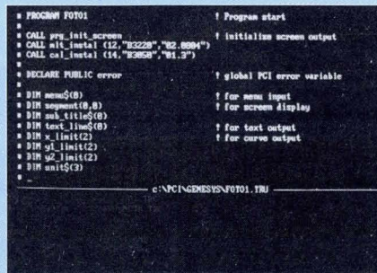
PCI-BASIC source code is generated with a single keystroke.
