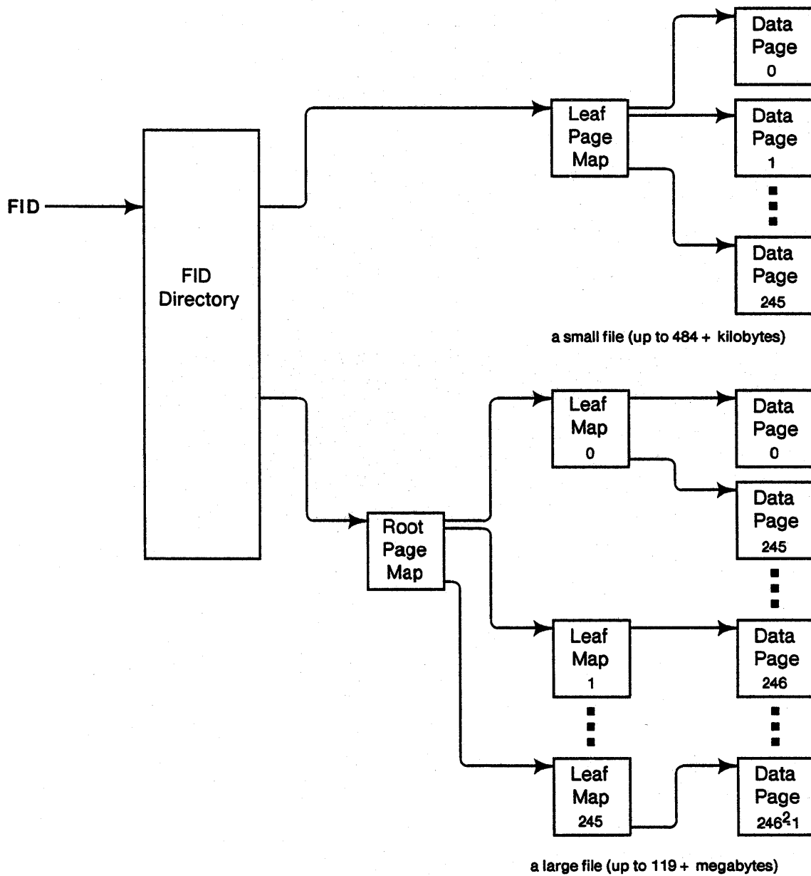
Figure 4. WFS file structure
