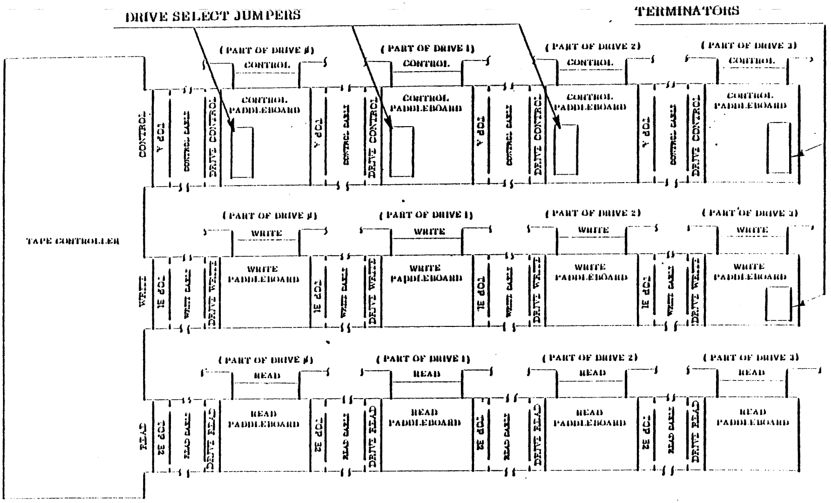
Figure 2-3. Tape Drive Daisy-Chain Connections
