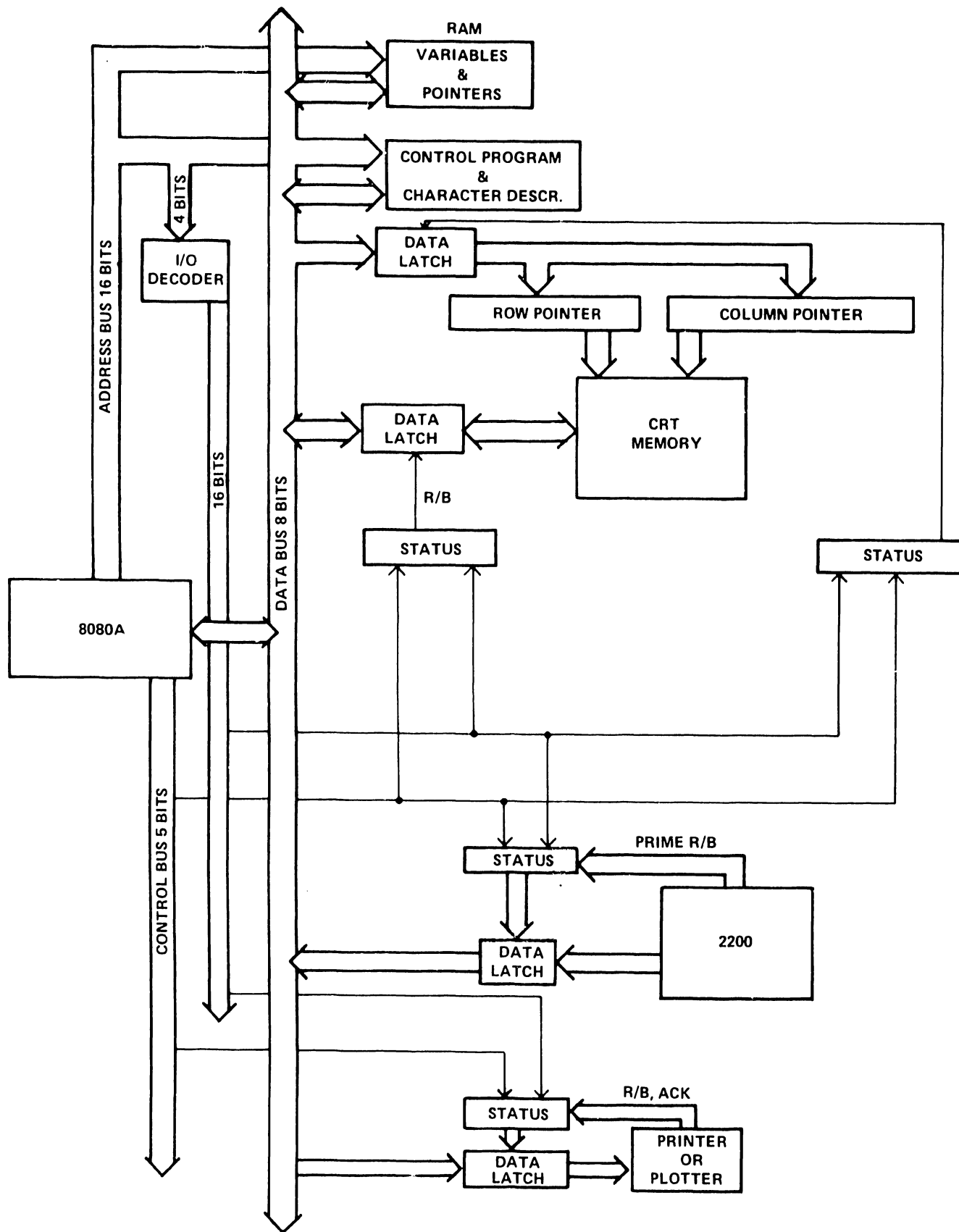
FIGURE 2 GRAPHICS CRT
