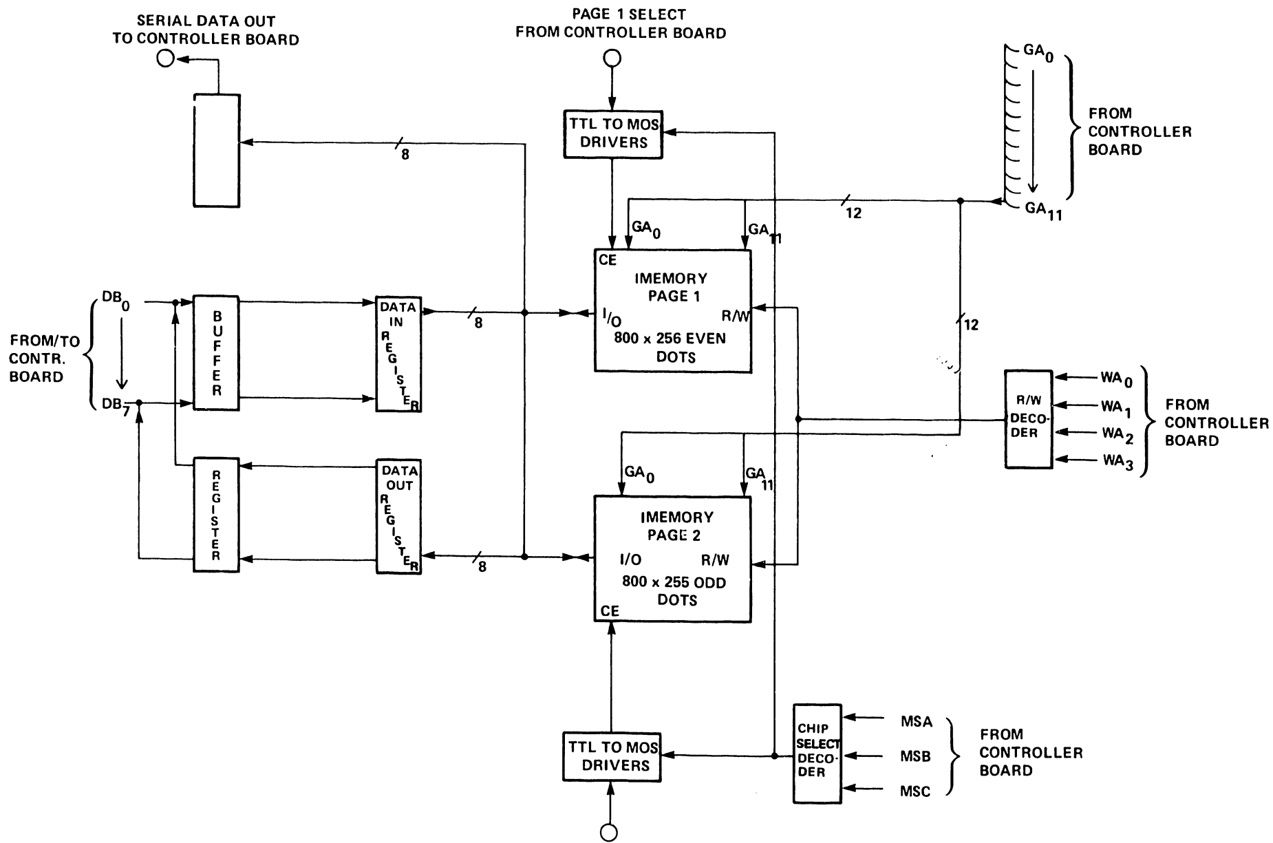
FIGURE 4 IMAGE MEMORY PCB #7298
