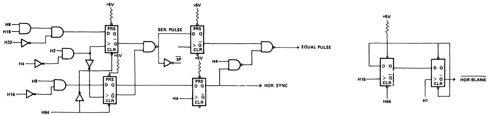
FIGURE 6 HORIZONTAL TIMING
