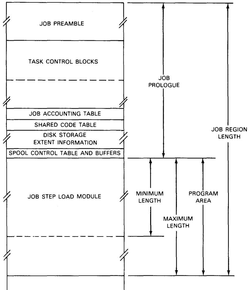
Figure 2—1. Job Region in Main Storage
