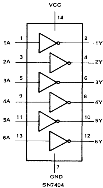
SN7404
