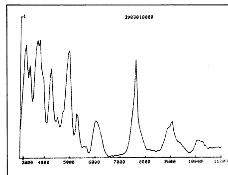
Fig. 8. Fast plot of sample spectrum 3903010000.
