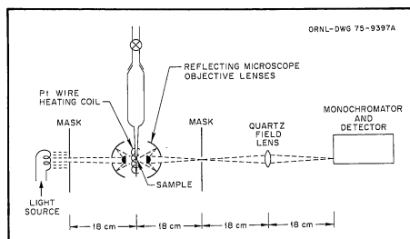
Fig. 1. Schematic diagram of microscope spectrophotometer.
