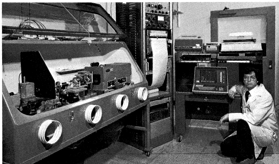
Fig. 2. Microscope spectrophotometer and Tektronix 4051 system.
