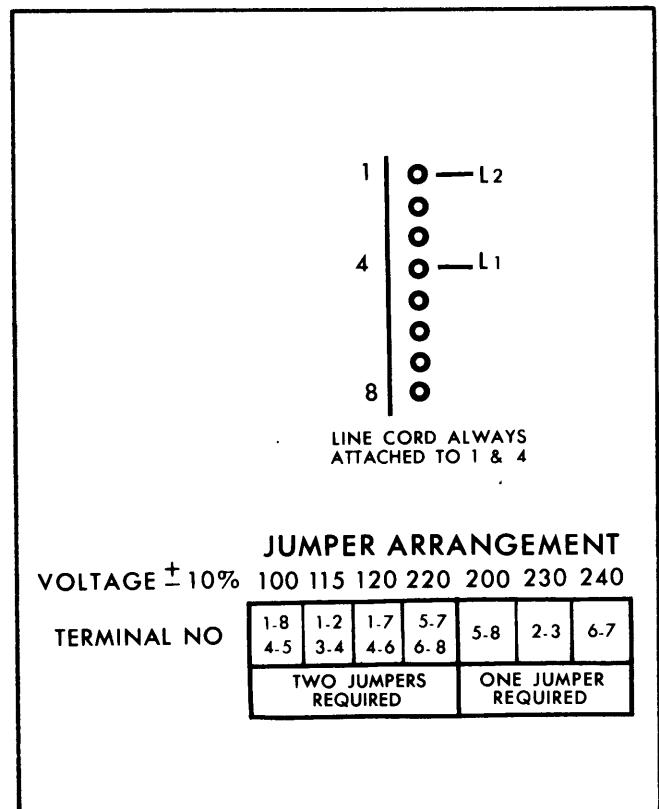
Fig. 2-6. Transformer Terminal jumper arrangement.
