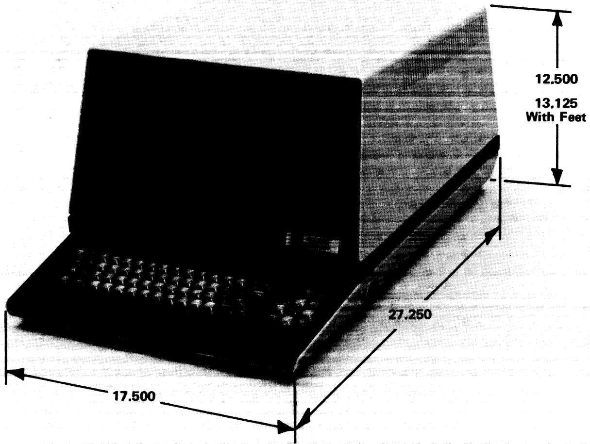
Fig. 2-4. Physical Dimensions.
