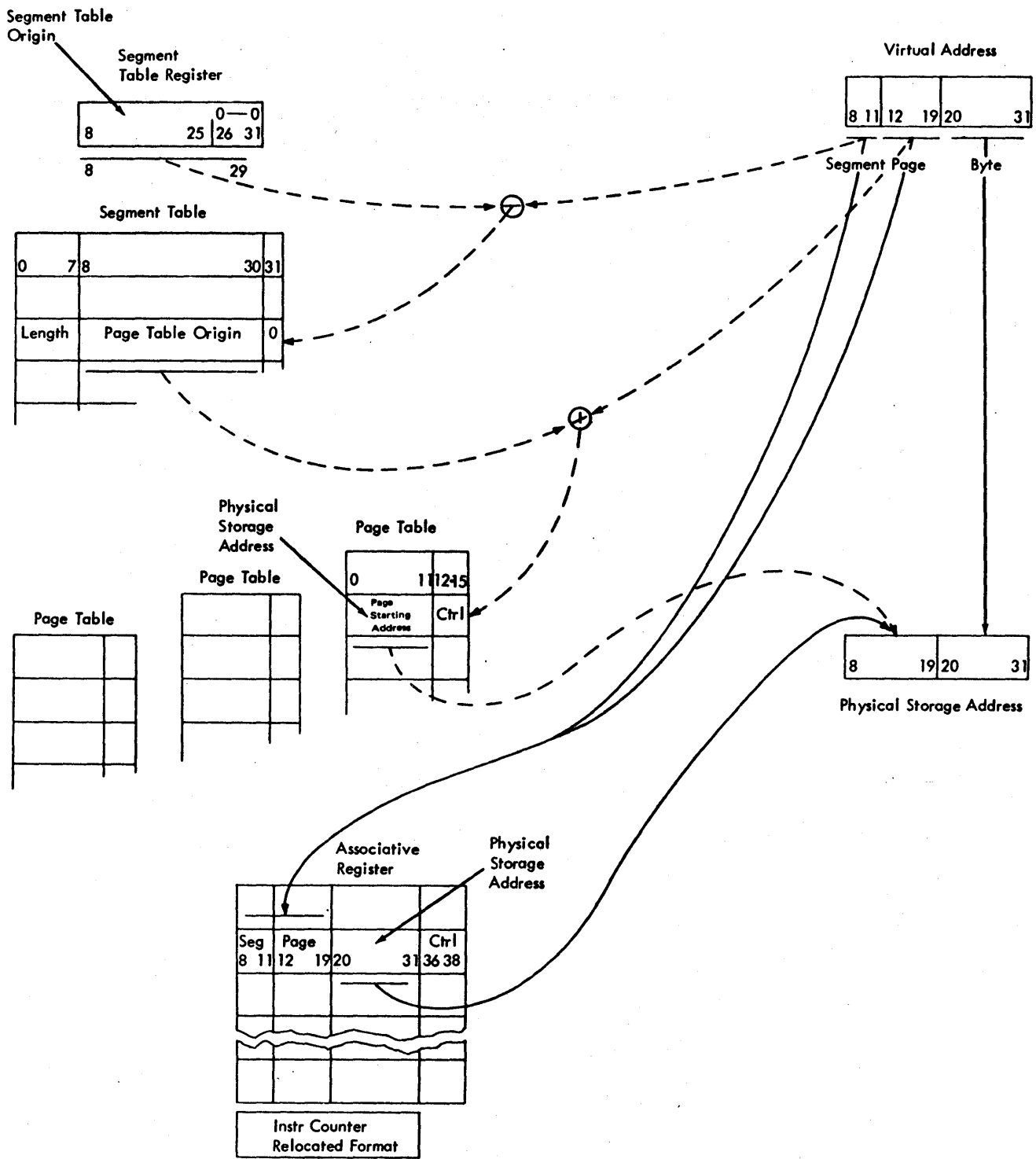
Figure 5. Data Flow for Dynamic Address Translation (24-Bit)
