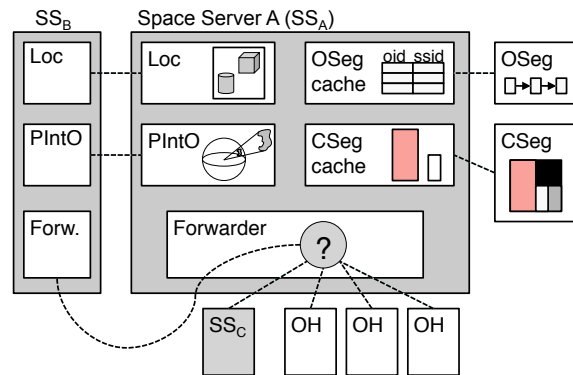
Figure 3: Space server internals. Dashed lines show network connections.
