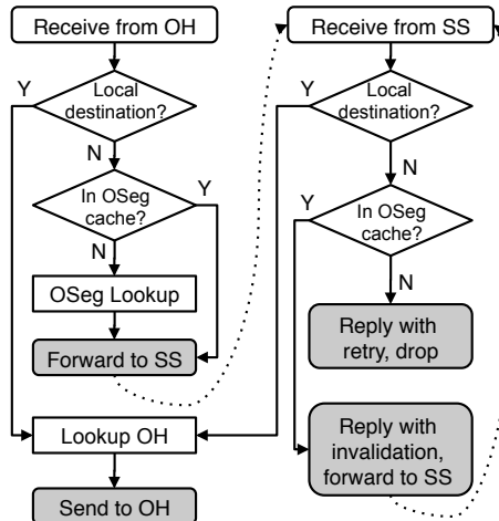
Figure 4: Flowchart of the object message forwarding pipeline in a Meru space server. The bottom of the right side is the case when a space server receives message for an object that has moved away.
