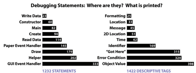
Figure 7. Analysis of the source code of 17 projects revealed that people place most of their debugging statements (printlns) in event handlers (GUI and R3). Many of the only statements tell the developer when the code “Got Here.” However, most are of object values specific to the particular application.
