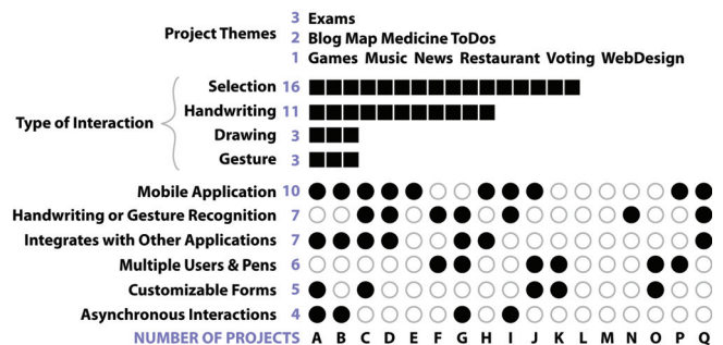
Figure 4. Summary of 17 class projects developed with R3. We see that R3 supported a variety of projects (though three dealt with university exams). Notice that while selection interactions were common (e.g., check a box), advanced interactions such as gestures were rare (e.g., draw a musical note). Notably, only four of the projects implemented asynchronous interactions, where ink and actions are batch processed once the user returns to their desktop.
