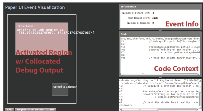
Figure 10. Building on debugging practices, R3 presents output on a 2D visualization of the paper UI. Here, the developer has interacted with the large paper region; its digital counterpart is highlighted. A panel displays the event code from the context of the region. Finally, showMe() displays output next to the region.
