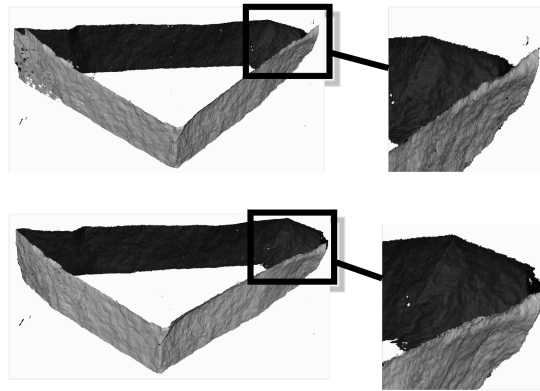
Figure 6. Global registration example showing the need for area-normalization. In the top image, the point-pairs were not normalized. The object has 3-4 meshes overlapping in all but one area (denoted with a square). This area contains only 2 overlapping meshes, and as illustrated in the zoomed image, the meshes have separated. The bottom image illustrates our result with area-normalization.
