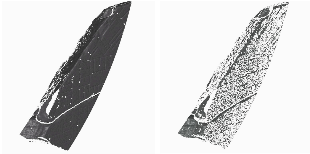
Figure 10. Sample scan demonstrating our filtering technique. The scan on the right is the filtered version of the scan on the left, where we filtered all vertices where the dot product between the normal and the scan direction was less than 0.65, which roughly corresponds to an angle of 50 degrees. As this figure demonstrates, much of the scan data is filtered out, meaning many of the vertices were scanned at an acute angle to the surface and were thus unreliable samples.
