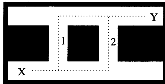
Figure 3.7: A map showing why the most likely state sequence may be different from the most likely states.
