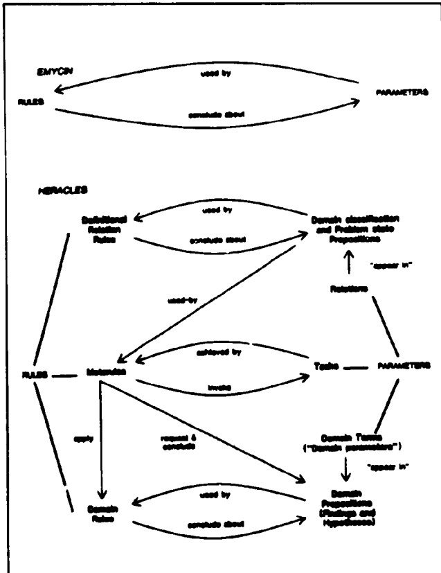
Figure 17. How Control Knowledge is Encoded in HERACLES. HERACLES is implemented as a specialization of MYCIN. Above is shown the original conception of domain parameters and rules. In HERACLES parameters are specialized as domain relations, control tasks, and domain terms, conditionally inferred and involved by rules. We use "relation" in the mathematical sense to refer to both predicates and functions. "Finding" and "hypothesis" formally classify the domain terms (for example, meningitis), and informally are used to refer to propositions in a situation-specific model; so, we say that "the patient has meningitis" is a hypothesis. Tasks are accomplished by an interpreter that applies metarules. Propositions used by metarule premises (such as (EXPLAINED-BY $F $H) appearing in Figure 16), can be inferred definitionally by rules or can be inferred by procedural attachment (for example, accessing Lisp structures). These propositions are both static and dynamic. They classify domain propositions and domain rules, as well as characterizing the problem-solving state (such as whether a hypothesis is in the differential or whether a task has been done yet). Additional relations that classify tasks are used by the task interpreter (not shown here). Metarule actions apply domain rules, request (from the user) or conclude domain propositions, or involve other tasks. In particular, the task FINDOUT uses all of these methods to infer domain propositions. In HERACLES all domain rules are applied directly by metarules rather than by back chaining. Only domain rules mention domain terms directly; other rules use variables.
