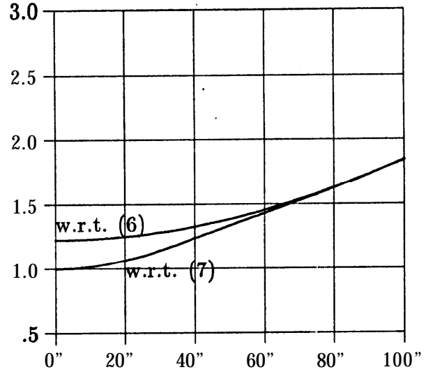
6b. "Optimum" \rho and \sigma versus \theta when \theta = -\phi for both smoothness measures.
