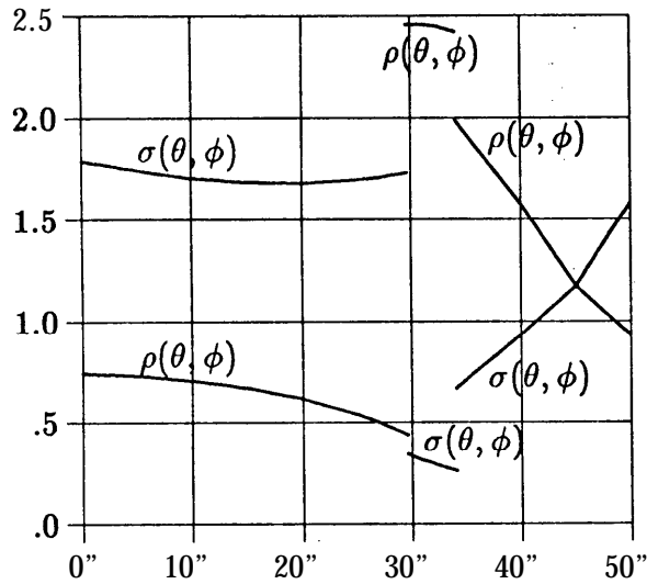
4a. The functions \rho(\theta, \phi) and \sigma(\theta, \phi) versus \theta for \phi = 90^\circ - \theta , minimizing the magnitude of curvature.
