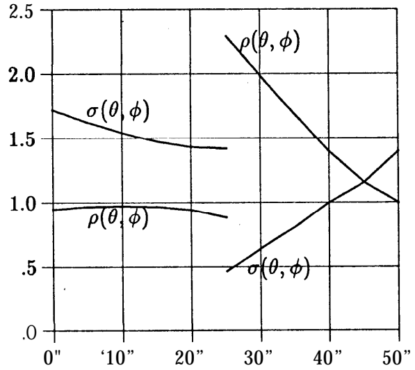
4b. The functions \rho(\theta, \phi) and \sigma(\theta, \phi) versus \theta for \phi = 90^\circ - \theta , minimizing the magnitude of curvature change.
