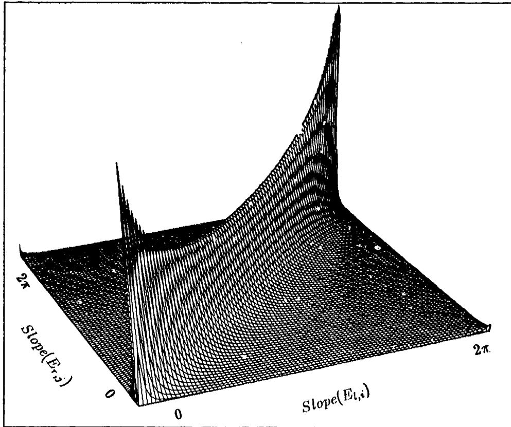
Edge angle probability density function (from [Arnold 1980]) Figure 4-6
