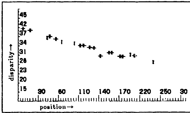
Edge correspondences (←→ preliminary edge matches < > subsequent edge matches) Figure 7-31
