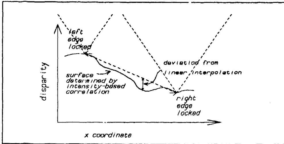
Intensity matching with both end points locked Figure 4-8
