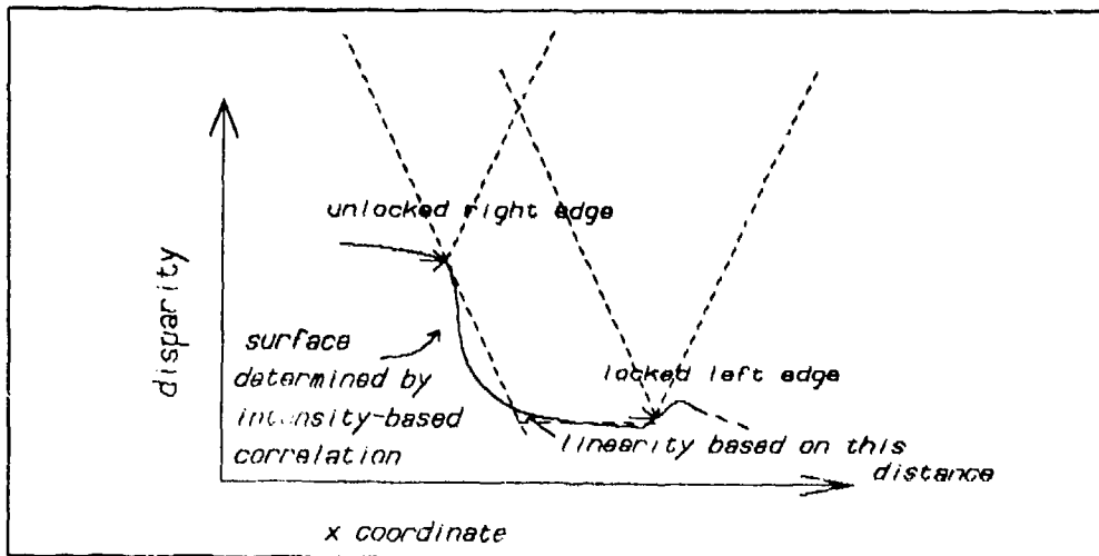
Intensity matching with one end point free Figure 4-9
