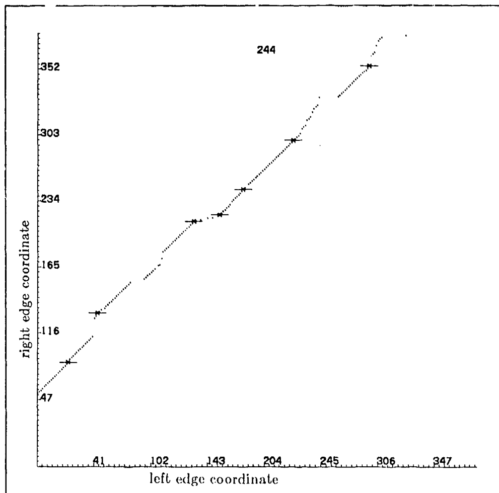
Edge and Intensity correspondences ( \leftarrow \rightarrow preliminary edge matches ) ( \leftarrow \rightarrow subsequent edge matches )
