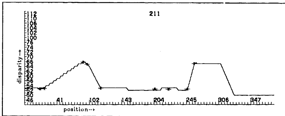
Interpolated disparities
