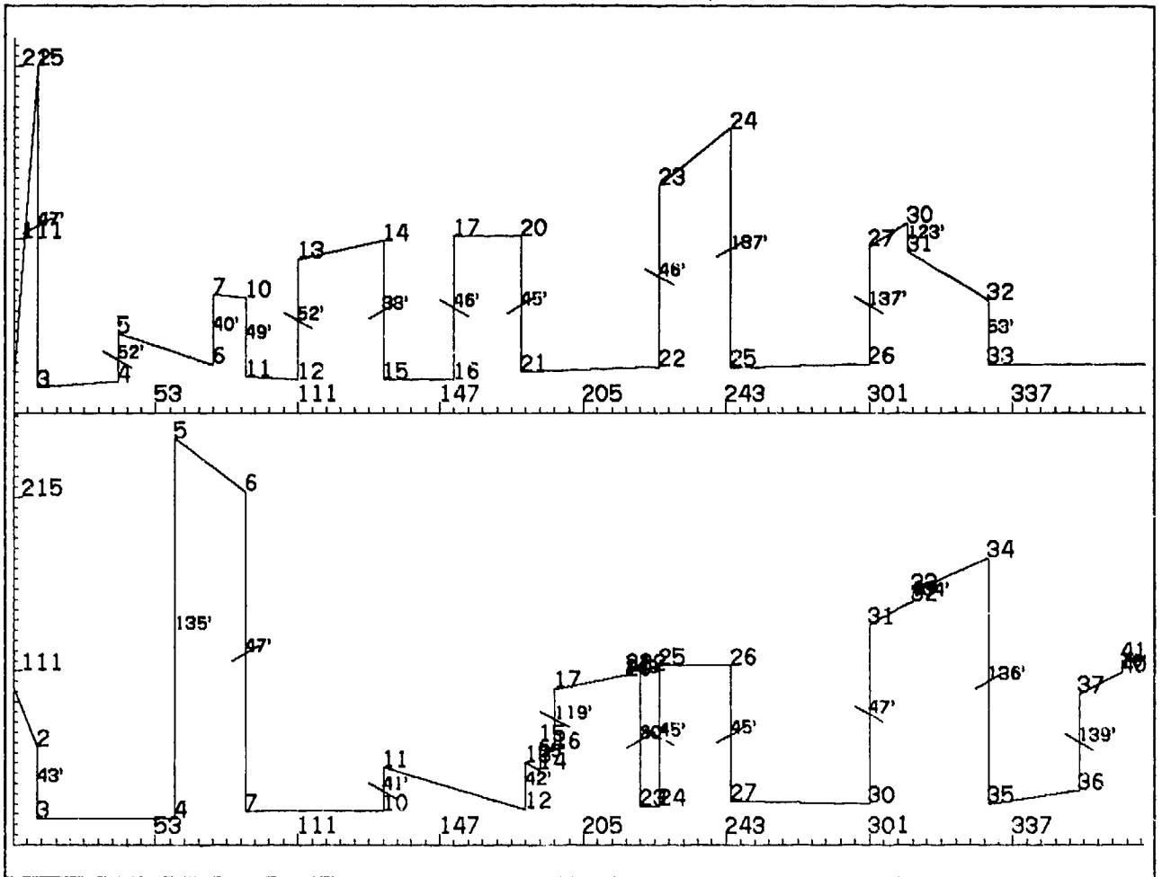
Edges of left and right image line 244 Figure 5-3
