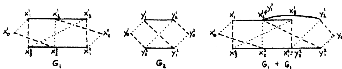
Figure 4. Concatenation
