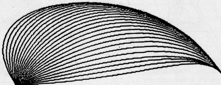
Figure 8. Same as Figure 7 but adjusted so that r' = \min\left(\frac{1}{2}, r\right) , s' = \min\left(\frac{1}{2}, s\right) .
