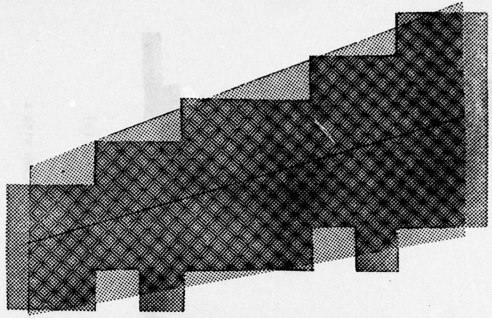
Figure 19. Failure of monotonicity due to independent rounding. (Rounding takes (w, x, y) into (\lfloor w \rfloor, \lfloor x - \delta(\lfloor w \rfloor) \rfloor, \lfloor y \rfloor) .)
