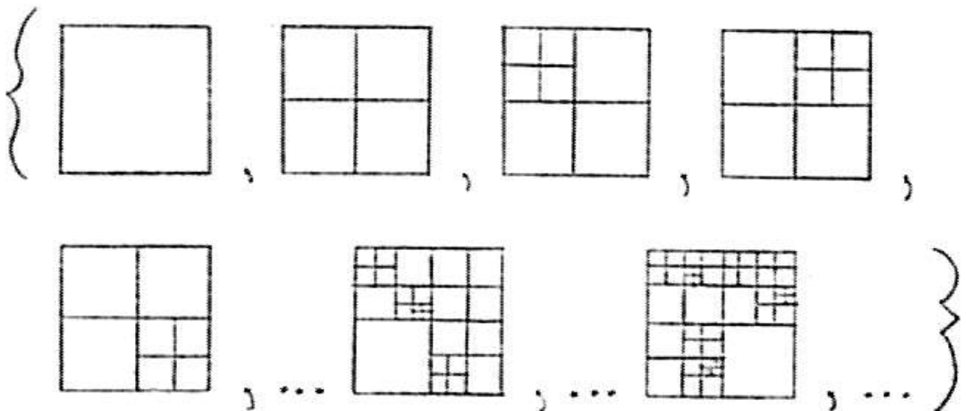
Figure 4c. The language defined by SG_1 used in serial.
