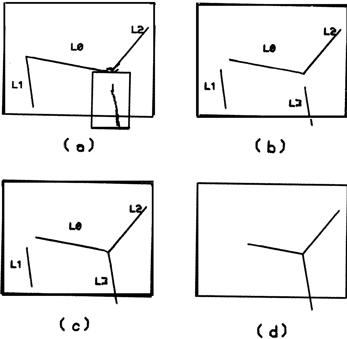
Fig. 7. Finding a three-sided corner with one low-contrast edge. (a) New edge points found in small window. (b) Lines. (c) Matching vertex formed. (d) Model of corner that was found. (Run time = 7 sec).
