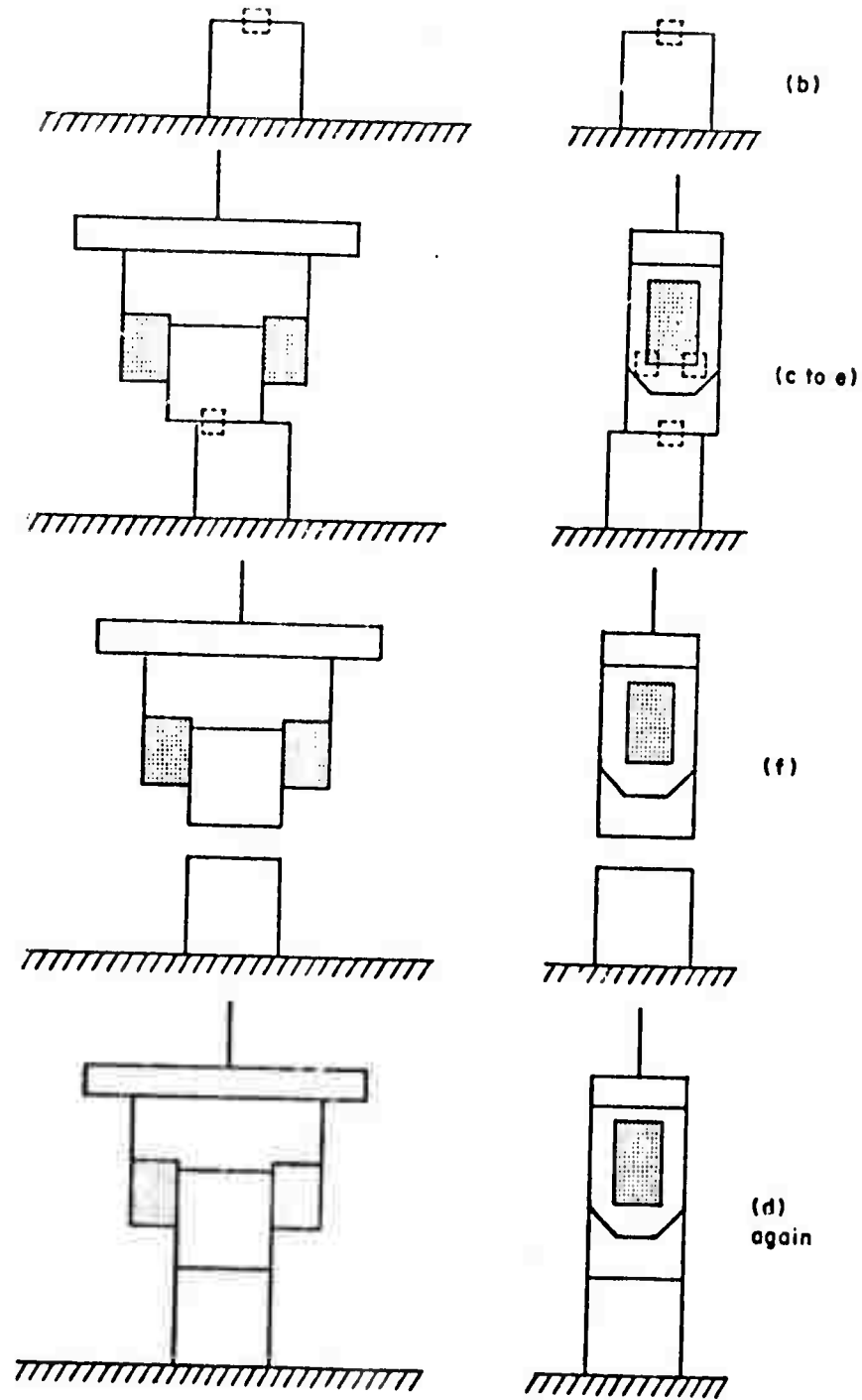
Fig. 4. STACKING TASK
