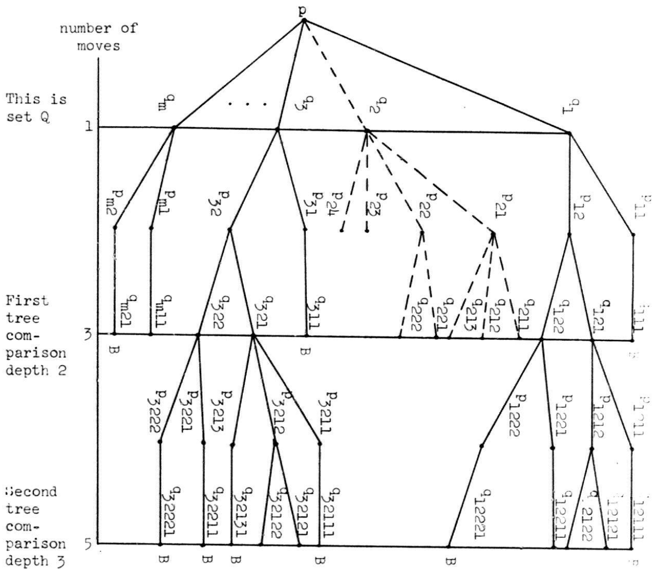
Figure 2.2. Example of Forcing Tree.
