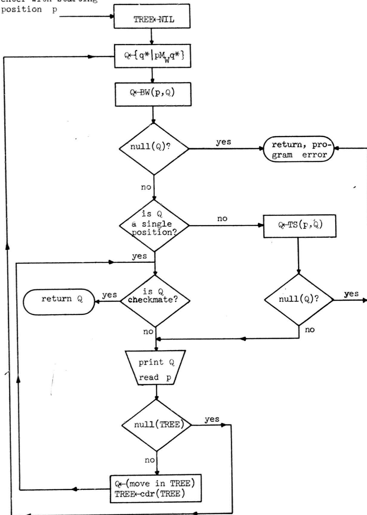
Figure 2.3. Main Program Flow.
