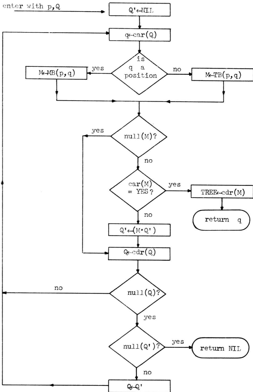
Figure 2.4. Function TS(p,Q) is the top level tree search function which starts the tree search going; calls the functions which follow the branches of the tree; returns the selected position and saves the branch in TREE if a decision is made; or starts again to extend the search one more level if no decision is made.
