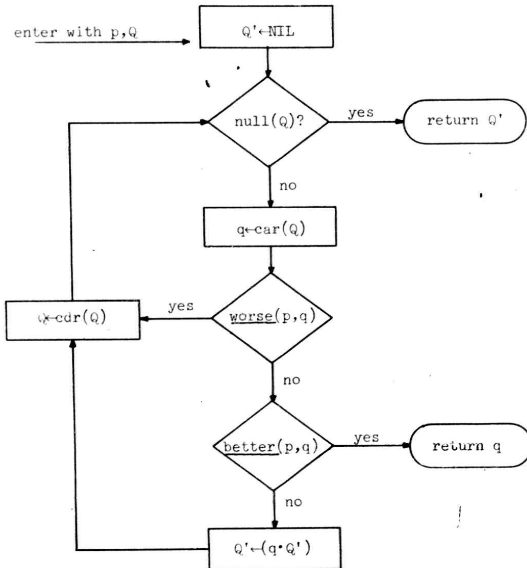
Figure 2.1. BW(p, Q)
