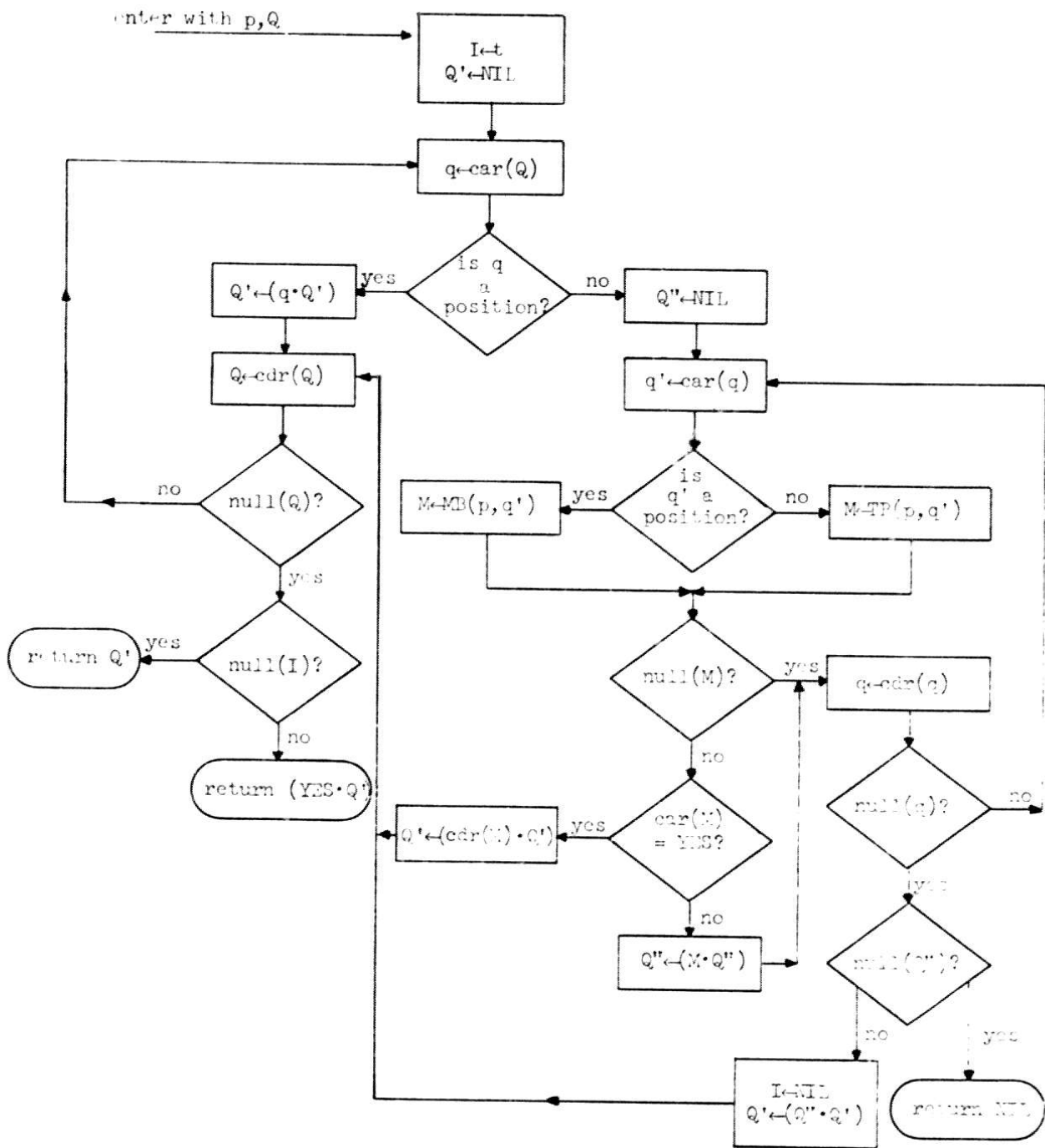
Figure 2.6. Function TB(p,Q) . Q is a list consisting of positions and of lists of positions. If an element of Q is a single position, then it was found to be better at the previous level. If the element is a list of positions, these are the non-worse positions from the previous level. Q contains an element for each black move in the position immediately above in the tree.
