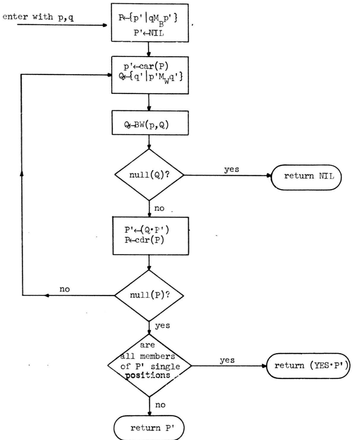
Figure 2.5. Function MB(p,q).q is a single position. Three values are returned. (1) NIL means that some black move from q cannot be answered. (2) YES·P' means that a better position is found for each black move from q . (3) P' means that for at least one black move no decision has been made.
