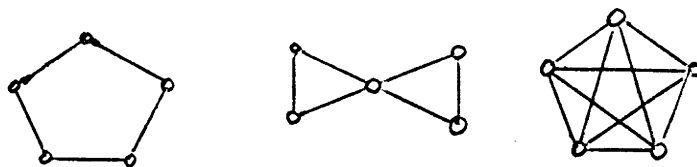
Nongraceful Graphs
