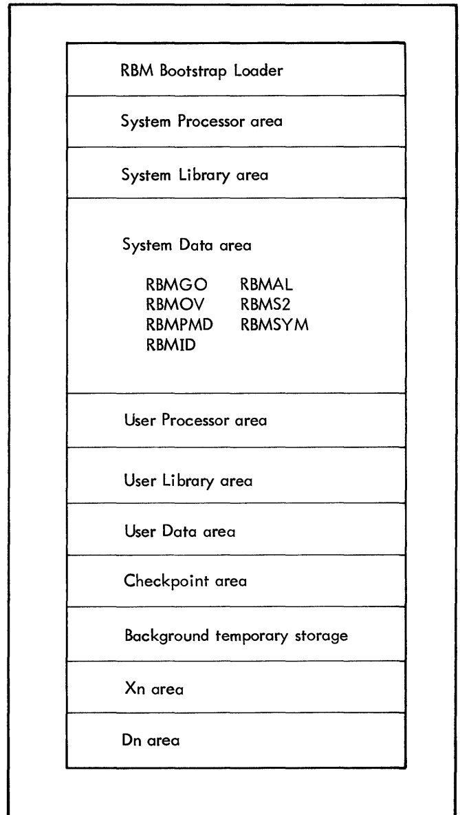
Figure 4. RAD Allocation
