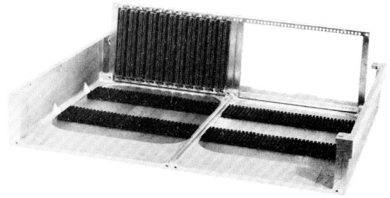
PHOTO 3 Inside view of the MICRAL with one Pluribus
