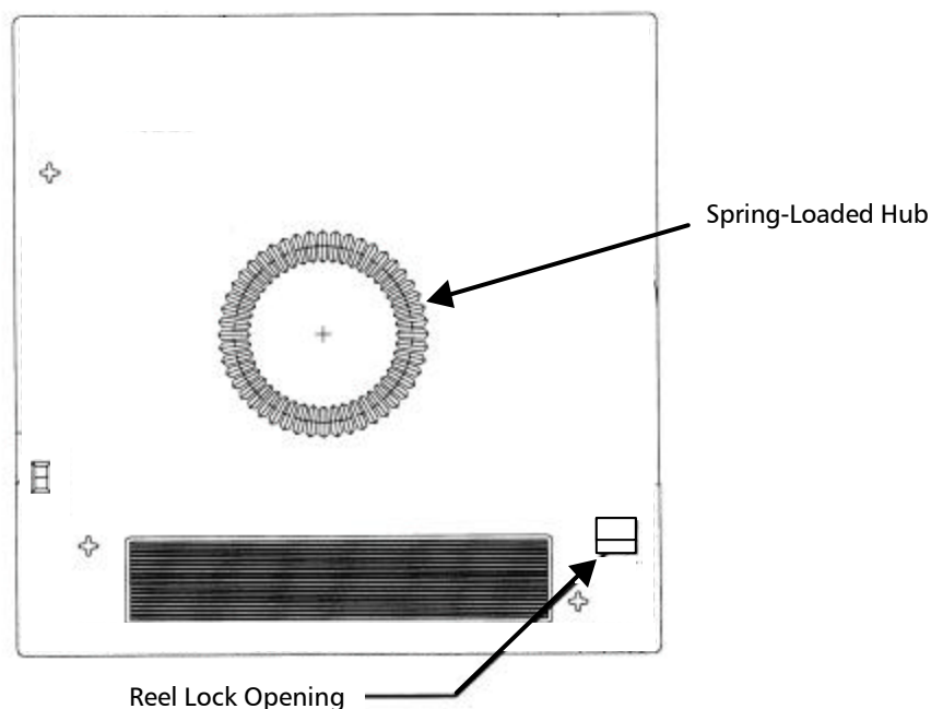
Figure D-2 Location of Reel Lock Opening and Spring-Loaded Hub on Bottom of DLTape Cartridge
