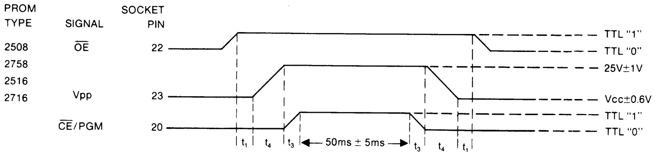
Figure 7-3. Programming Waveforms for Dynamic Test
