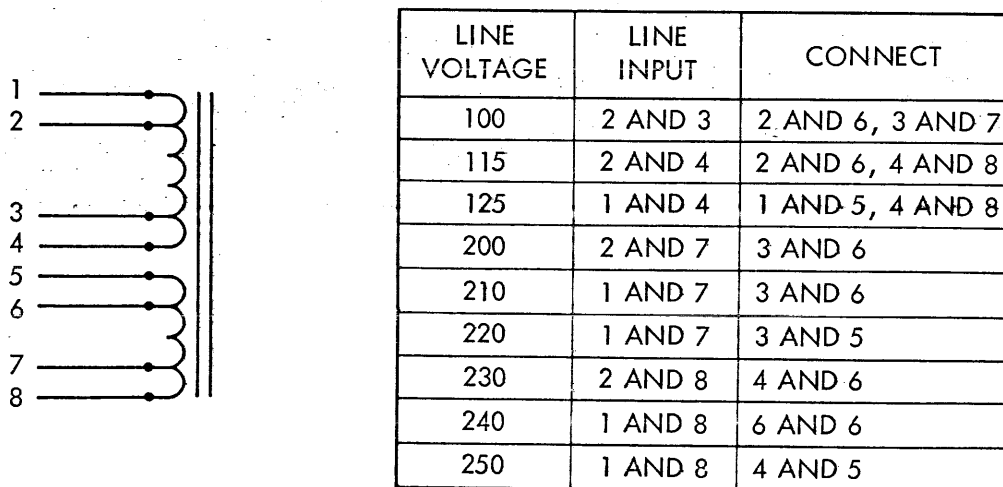
Figure 2-1. Transformer Primary Connections
