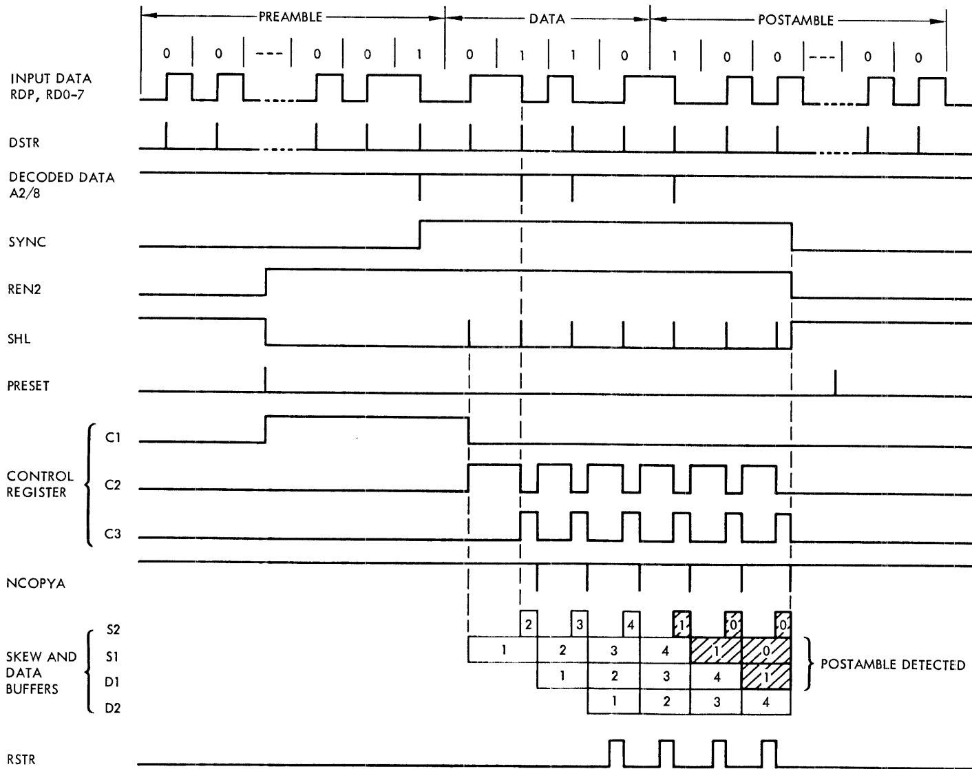
Figure 5-18. Data Buffering
