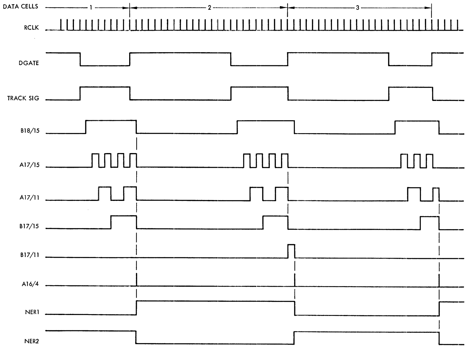
Figure 5-19. Tracking Control Waveforms
