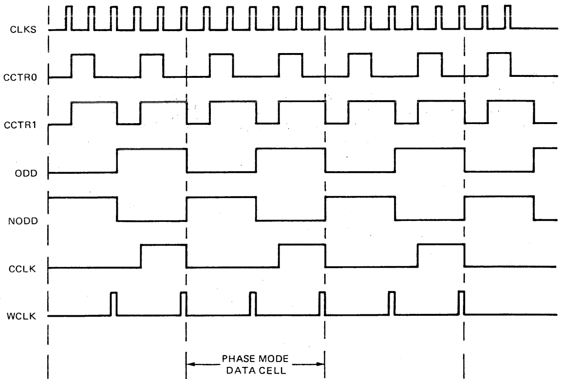
Figure 5-8. Clock Waveforms
