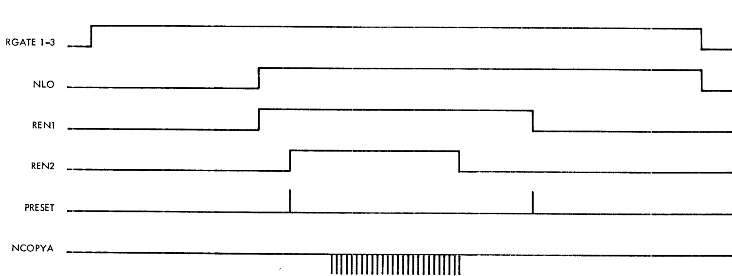
Figure 5-20. Control Signals to Data Channels
