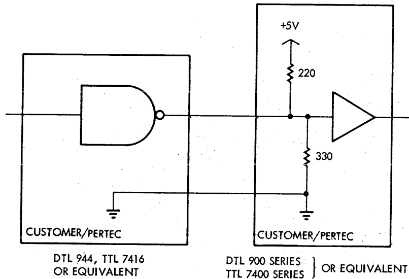
Figure 1-3. Interface Configuration
