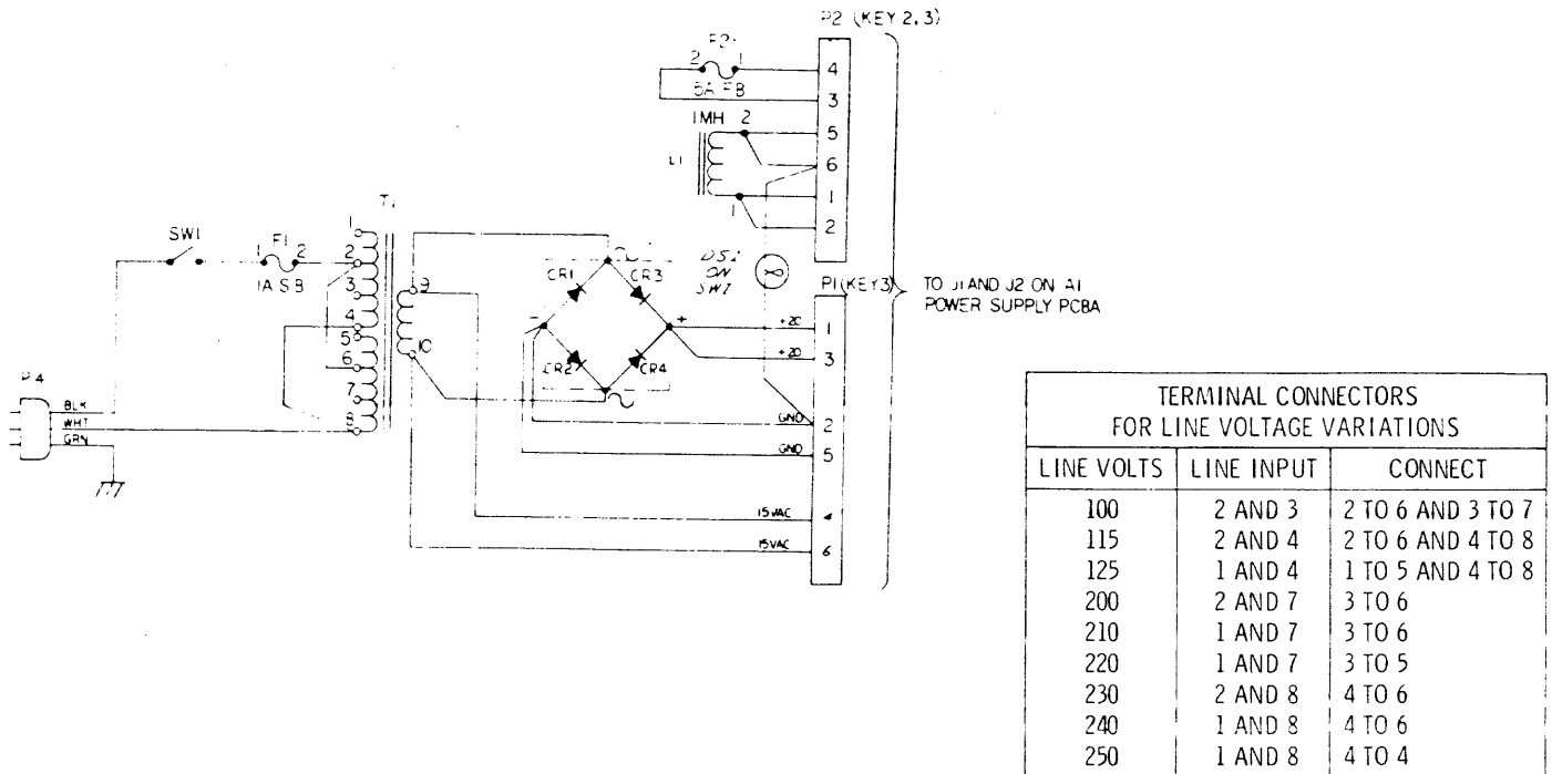
Figure 5-3. Chassis Mounted Power Supply Components
