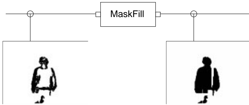
Figure 4-27: VsMaskFill
