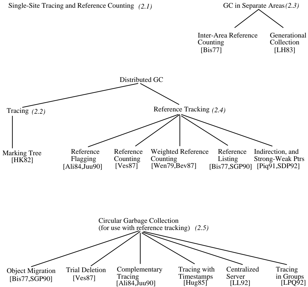
Figure 2-1: Techniques discussed in this chapter
