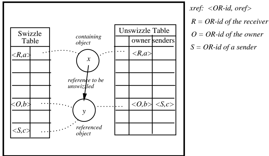
Figure 5-2: The front end remembers all xrefs associated with an object.
