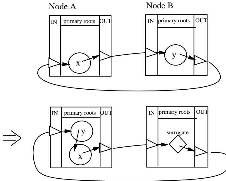
Figure 2-15: Treating migration using surrogates does not consolidate cycles by itself.
