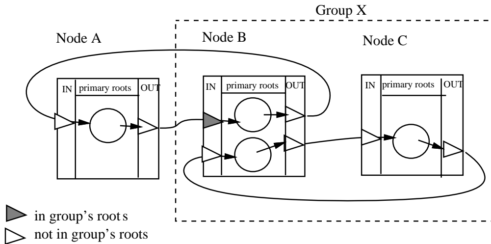
Figure 2-17: A group-wide tracing collects cycles lying within the group.
