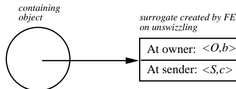
Figure 5-4: The surrogate sent to the coordinator contains xrefs at both the owner and the sender.
