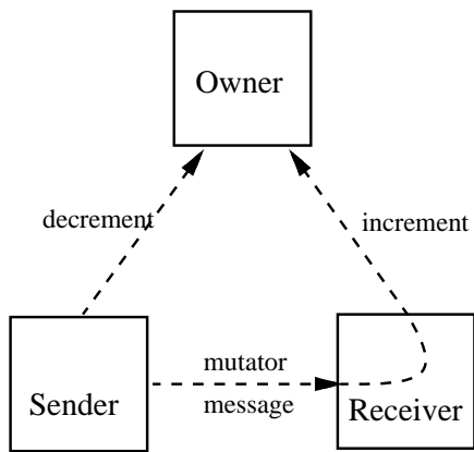
(i) Possible race condition
