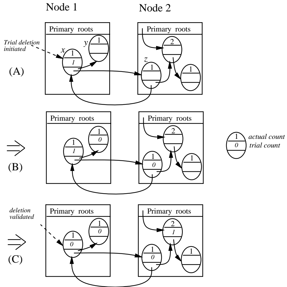
Figure 2-16: Trial deletion to detect circular garbage
