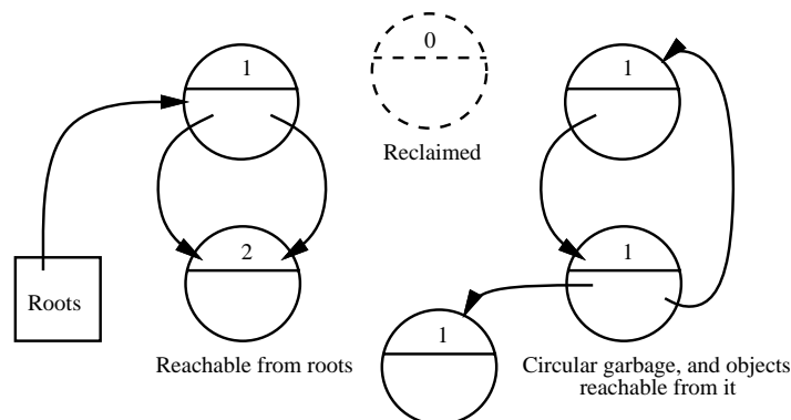
Figure 2-2: Reference Counting
