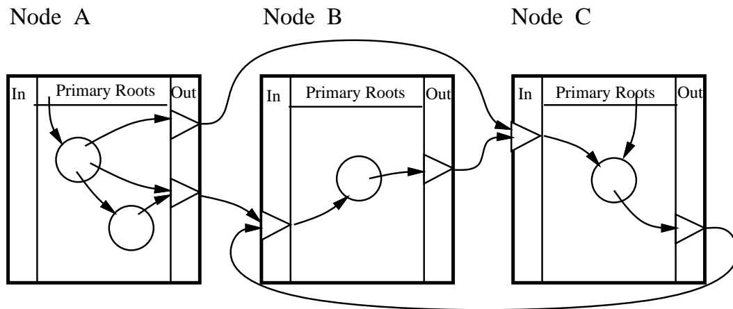
Figure 2-7: Inlists and outlists track inter-node references.
