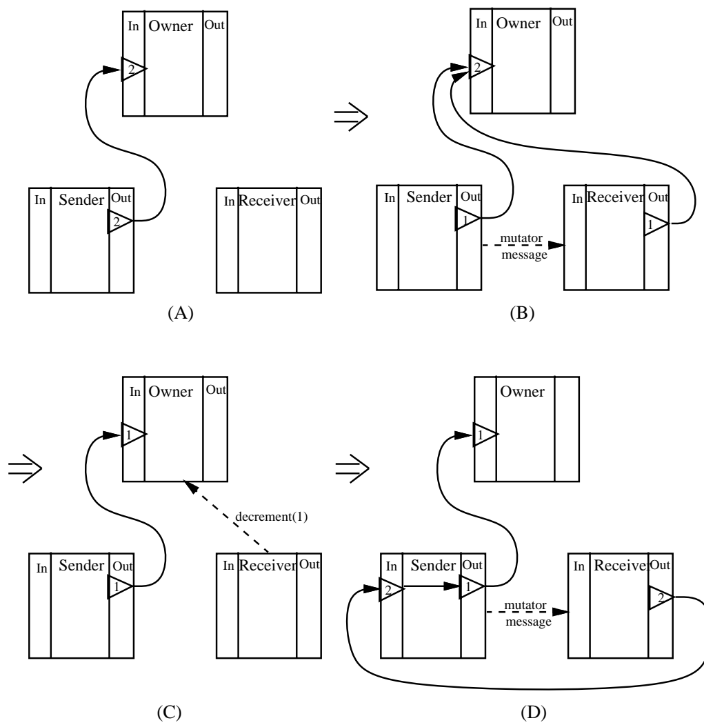
Figure 2-10: Weighted reference counting
