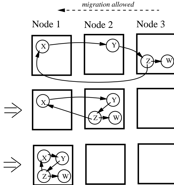
Figure 2-14: Consolidation of distributed circular garbage into one node
