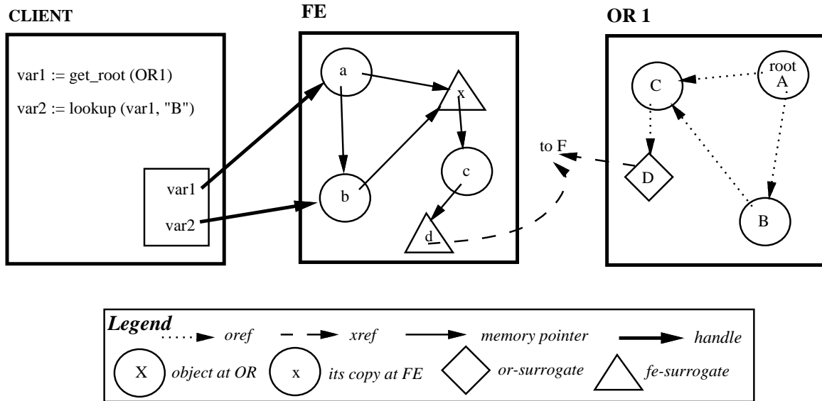
Figure 3-4: The client accesses objects at the front end through handles
