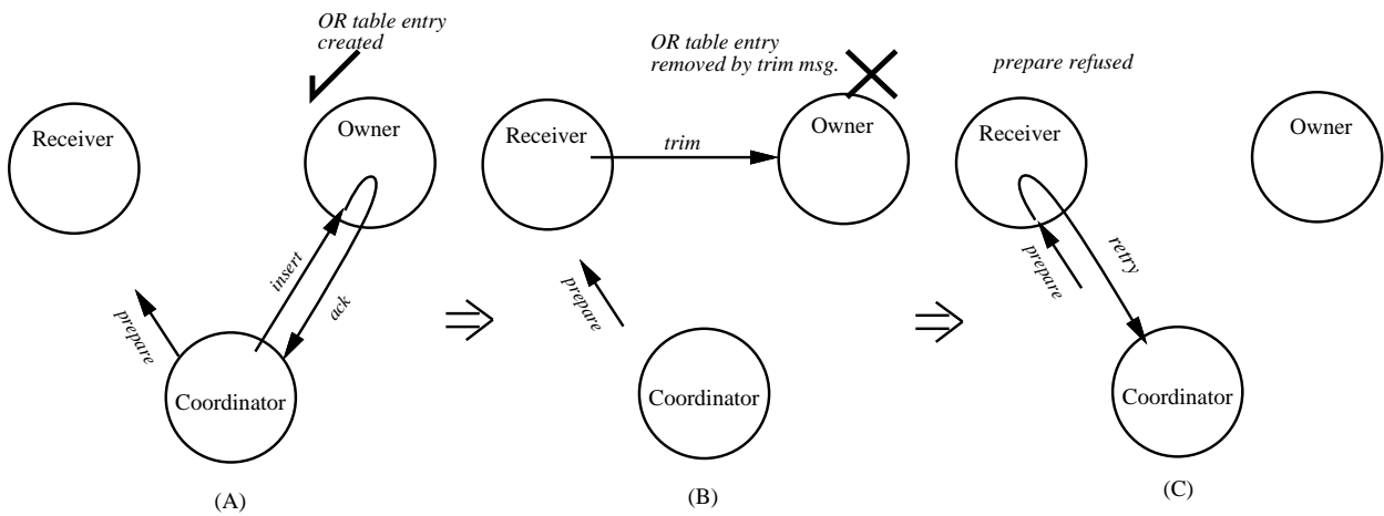
Figure 5-7: The trim message deletes an entry it did not account for.
