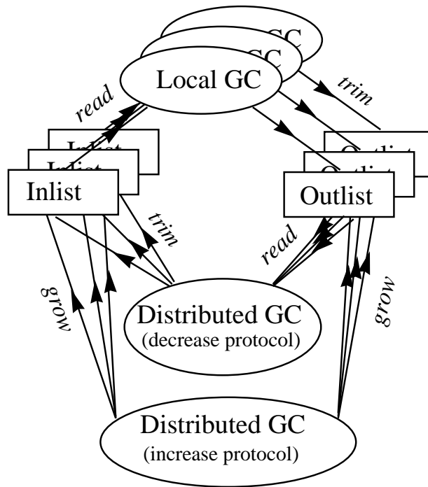
Figure 2-8: The roles of local and distributed GC in reference tracking
