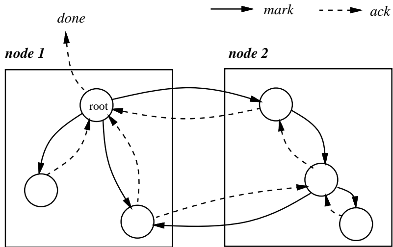
Figure 2-3: Marking-Tree for termination detection
