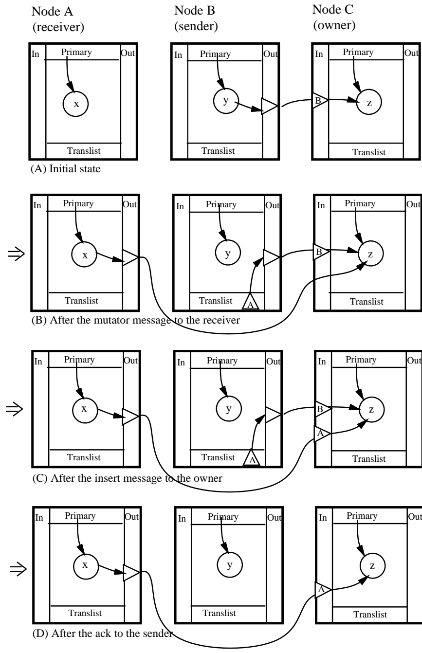
Figure 2-11: A translist entry exists until the delivery of the asynchronous insert message is confirmed.
