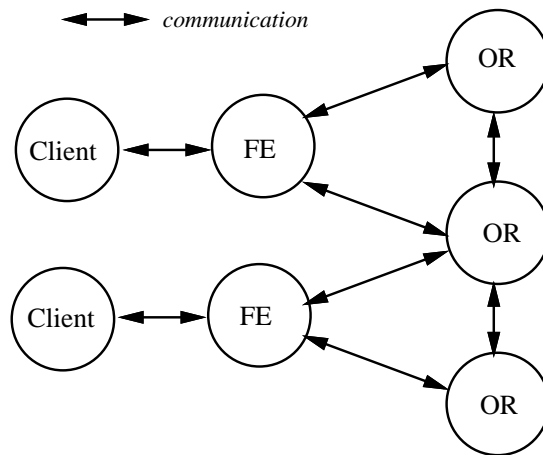
Figure 3-1: A configuration of clients, front ends, and object repositories in Thor.
