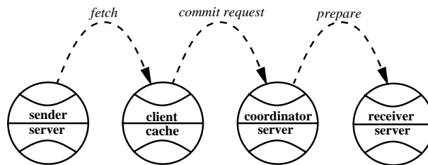
(B) Mutator messages in a client-server transactional system.
