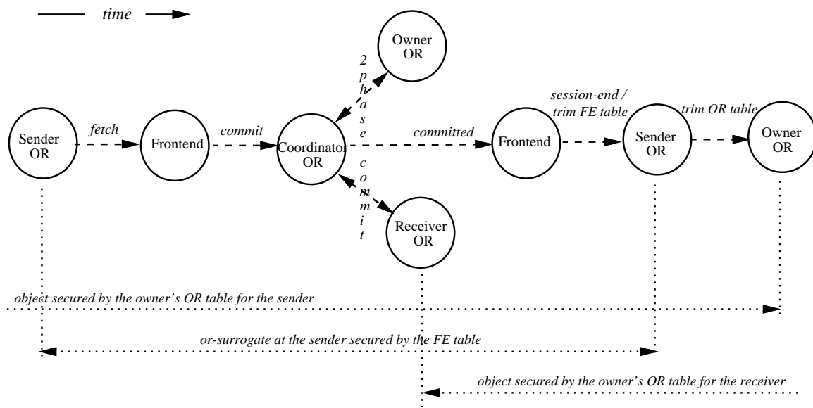
Figure 4-3: The overall plan: How objects with references in transit are protected.
