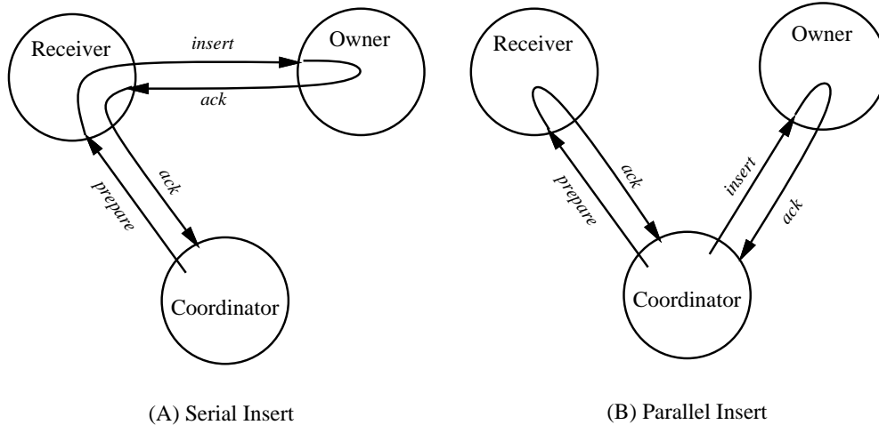
Figure 5-1: Two Insert Protocols
