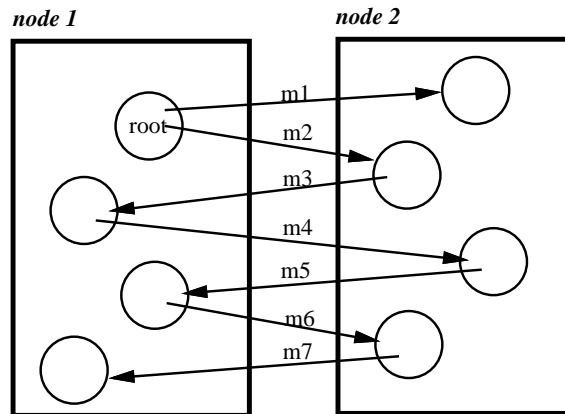
Figure 2-4: A chain of remote references results in a series of marking messages.
