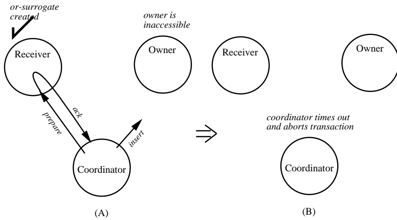
Figure 5-8: An unconfirmed or-surrogate may not have a matching OR table entry.
