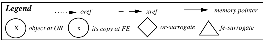
Figure 3-2: Inter-node references between ORs and Front Ends
