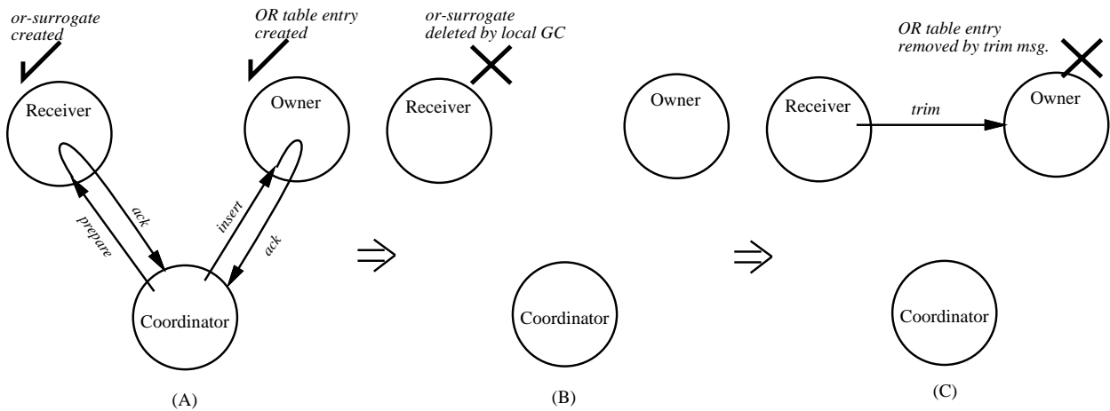
Figure 5-6: The trim message deletes a useless OR table entry.
