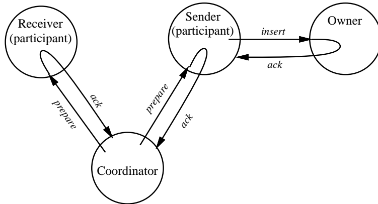
Figure 5-3: The sender sends an asynchronous insert message to the owner.
