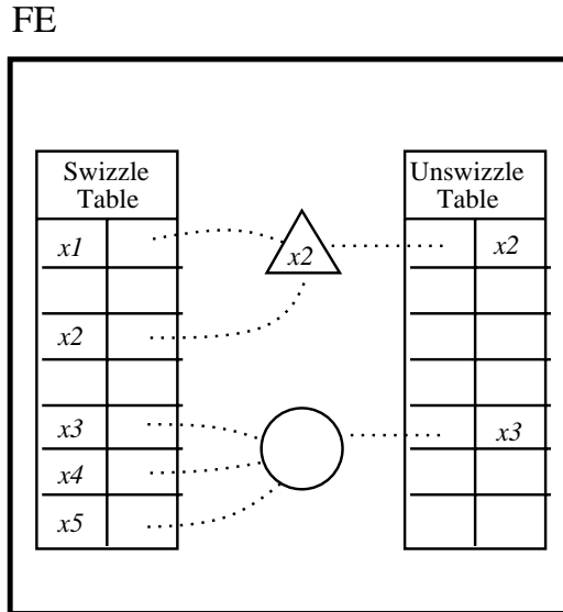
Figure 3-3: Swizzle table and unswizzle table
