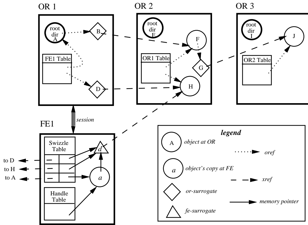
Figure 4-1: OR tables and FE tables protect objects accessible from primary roots.
