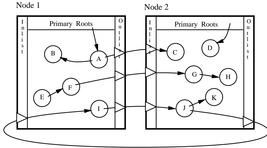
Figure 1-2: Garbage in a distributed object graph
