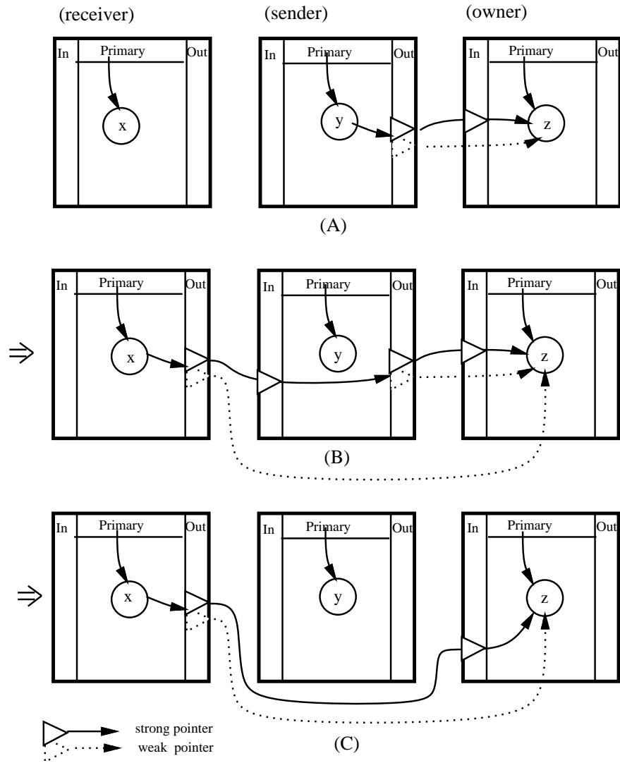
Figure 2-12: Indirection and strong-weak pointers
