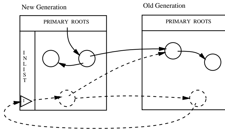
Figure 2-6: Generational collection collects inter-area circular garbage.
