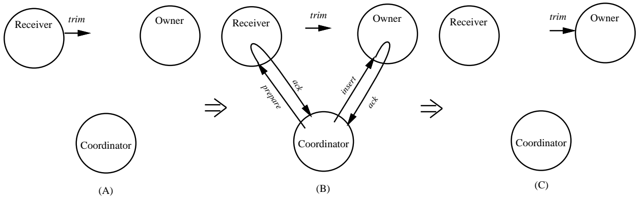
Figure 5-5: Race condition between insert and trim messages in the parallel insert scheme
