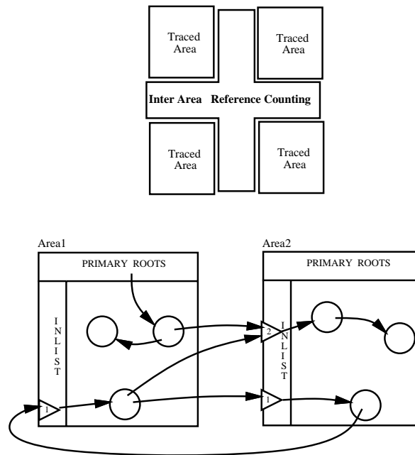
Figure 2-5: Inter-area Reference Counting
