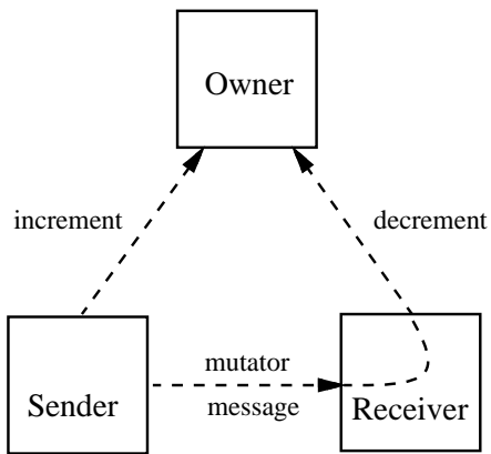
(i) Possible race condition
