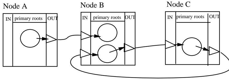
Figure 2-13: Collection of a cycle should not require all nodes to cooperate
