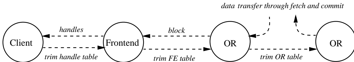
Figure 4-2: GC interaction between the client, the front end, and the ORs
