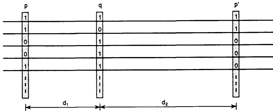
Figure 4-5: An interrupting module q on the first 0-interval of the highest arbitration priority p . There is another module p' with the same first two intervals as p on the other side of q .
