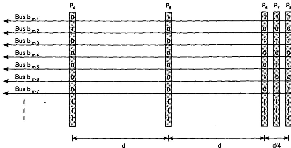
Figure 4-4: The arrangement of the five modules in set A that are responsible for creating the first “ping-pong wave form”, and for receiving the second “ping-pong wave form” and generating the third “ping-pong wave form”. The spaces between p_4 and p_5 , between p_5 and p_6 , and between p_6 and p_7 contain no other arbitrating modules. The space between p_7 and p_8 may contain other arbitrating modules for generation of future odd-indexed “ping-pong wave forms”.
