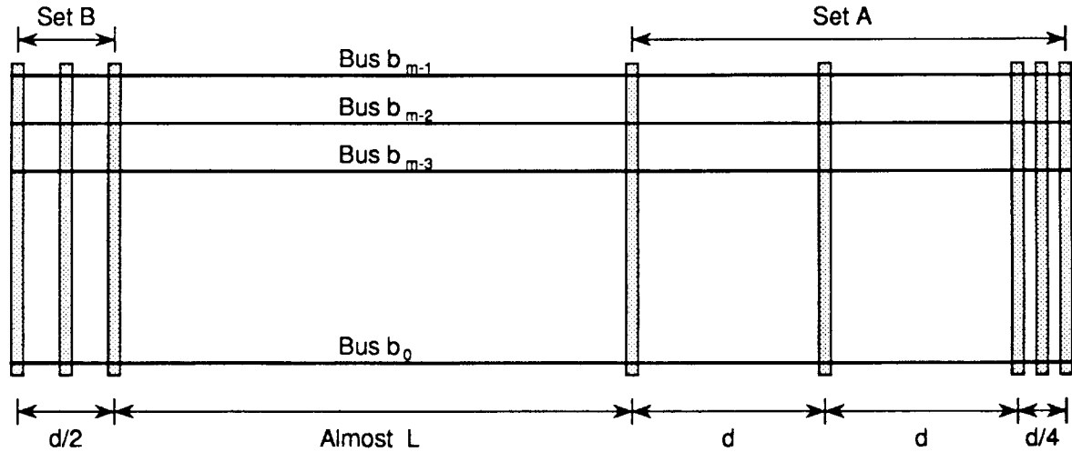
Figure 4-1: High level partitioning of the selected arbitrating modules into sets A and B . With a parameter d (to be determined later), the total length of set A is 9d/4 , the total length of set B is d/2 , and the distance between the two sets is almost L , such that d \ll L .
