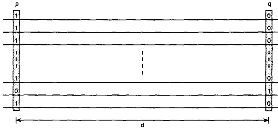
Figure 4-7: Linear arrangement of 2 modules very close to the two ends of the bus lines. The arbitration process on this arrangement asymptotically takes 3 units of bus-propagation delay.
