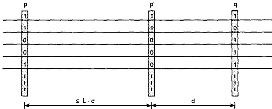
Figure 4-6: An interrupting module q on the first 0-interval of the highest arbitration priority p . All the arbitrating modules with the same first two intervals as p are on the same side of q .
