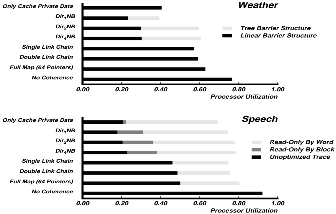
Figure 5-2: System-level optimizations.
