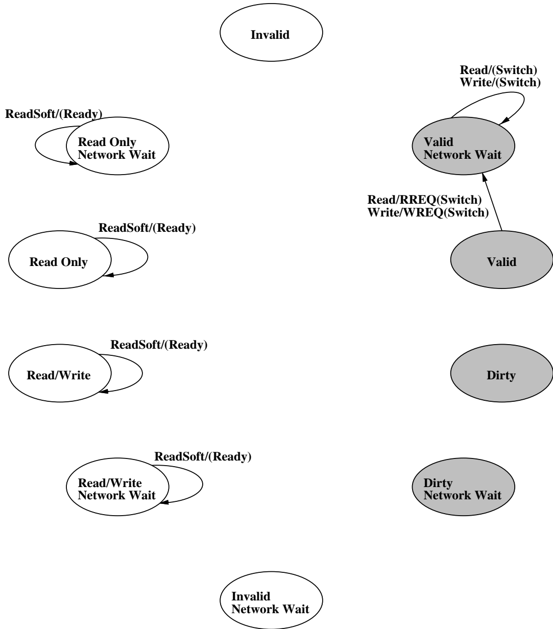
Figure B-2: Cache state transitions for processor requests when the tag matches, hardware/software coherence interaction.
